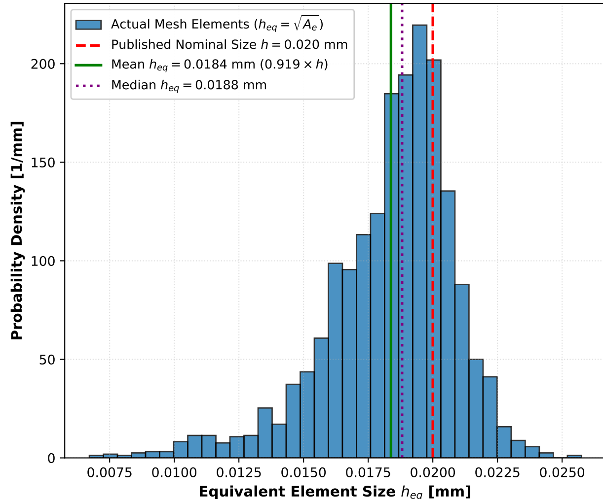
Element Size Distribution vs Published Specification (Pandey & Kumar 2025: h = 0.02 mm Global)
