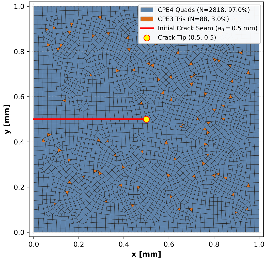
Canonical 2,906-Element Coarse Mesh Topology (Global Nominal Sizing h = 0.02 mm)
