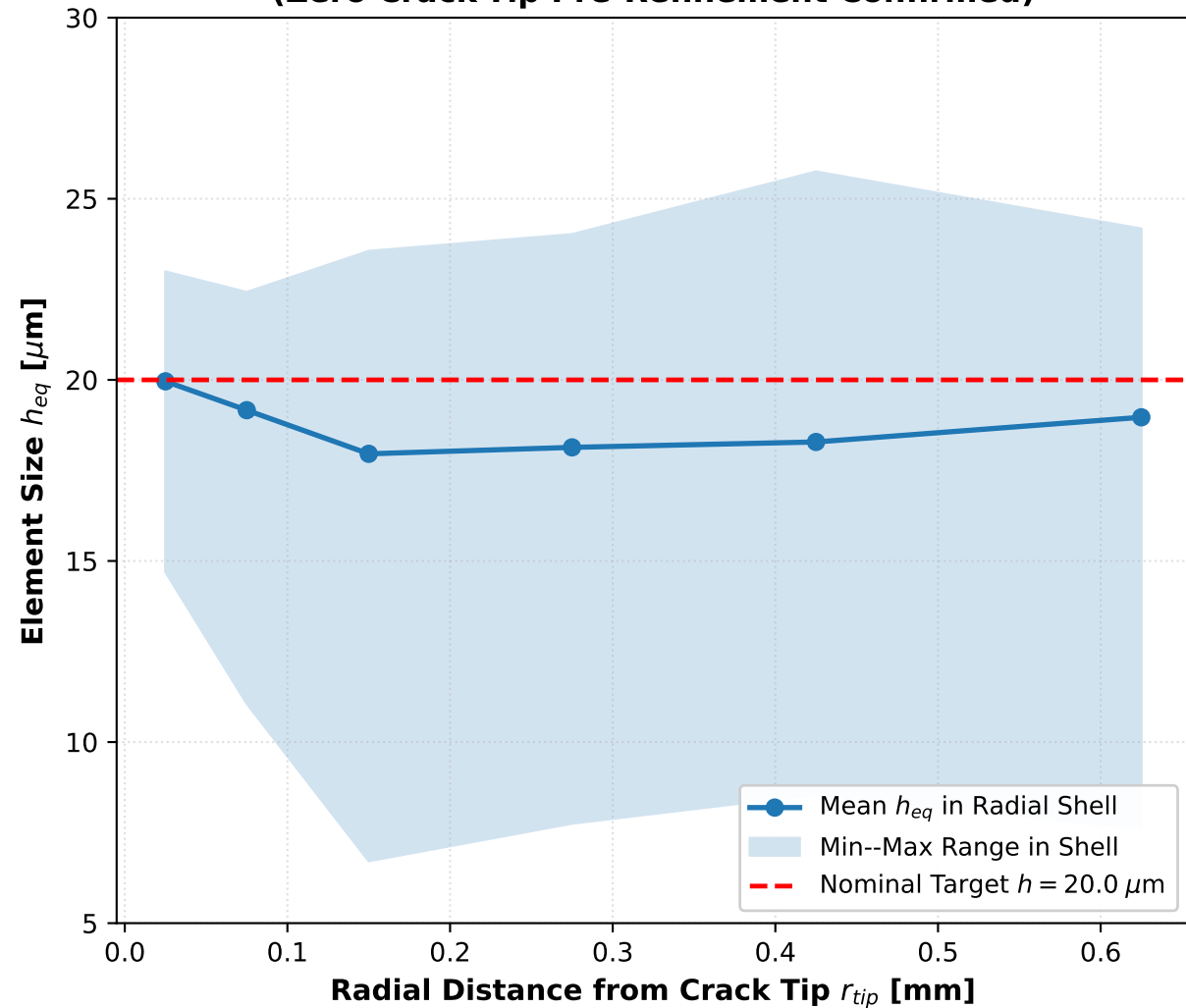
Radial Sizing Profile from Crack Tip (0.5, 0.5) (Zero Crack-Tip Pre-Refinement Confirmed)
