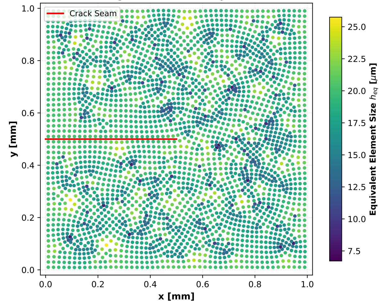
Spatial Map of Element Sizing h_{eq}(x, y) (Demonstrating Global Uniformity Across Domain)
