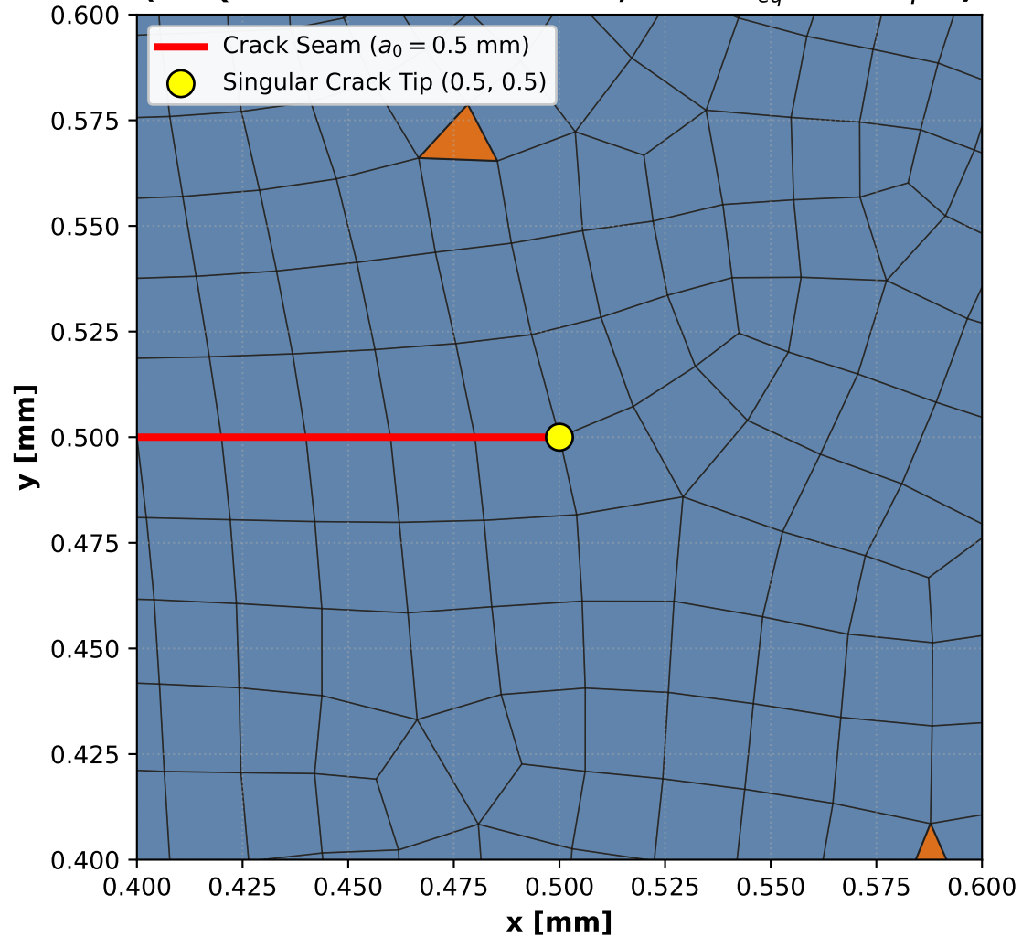
Crack-Tip Element Topology Closeup ( r \leq 0.10 mm) (20 Quads within r < 0.05 mm, Mean h_{eq} = 19.96 \mu\text{m} )
