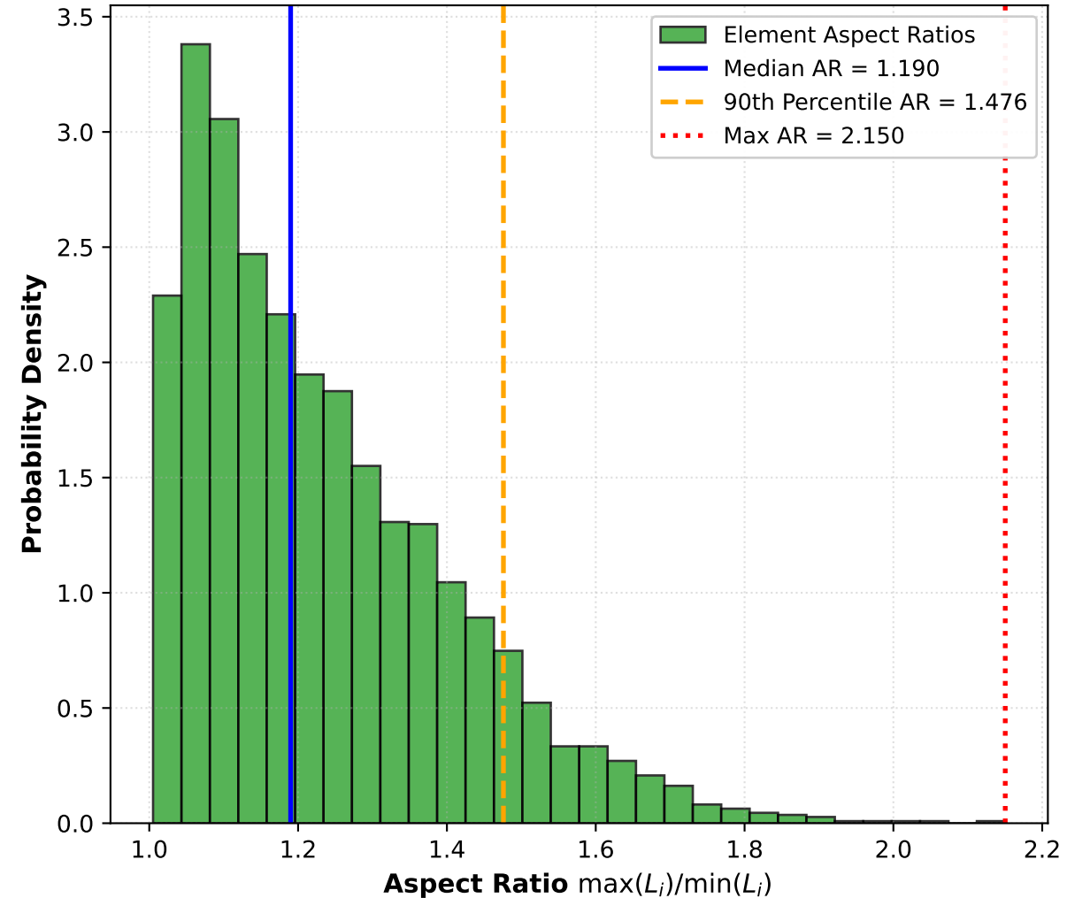
Element Shape Quality: Aspect Ratio Distribution (99% Elements with AR < 1.75; Low Distortion)
