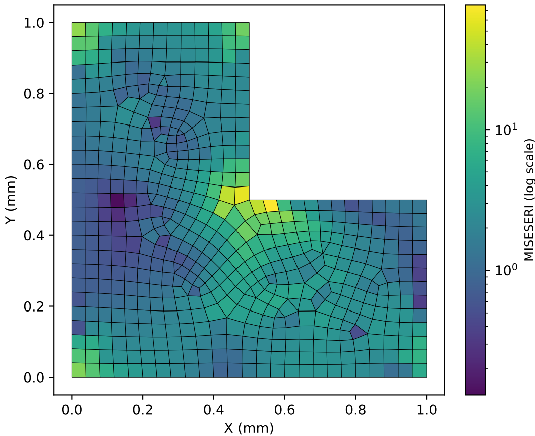
(a) Coarse Mesh & Raw MISESERI Field (True Element Polygons)
