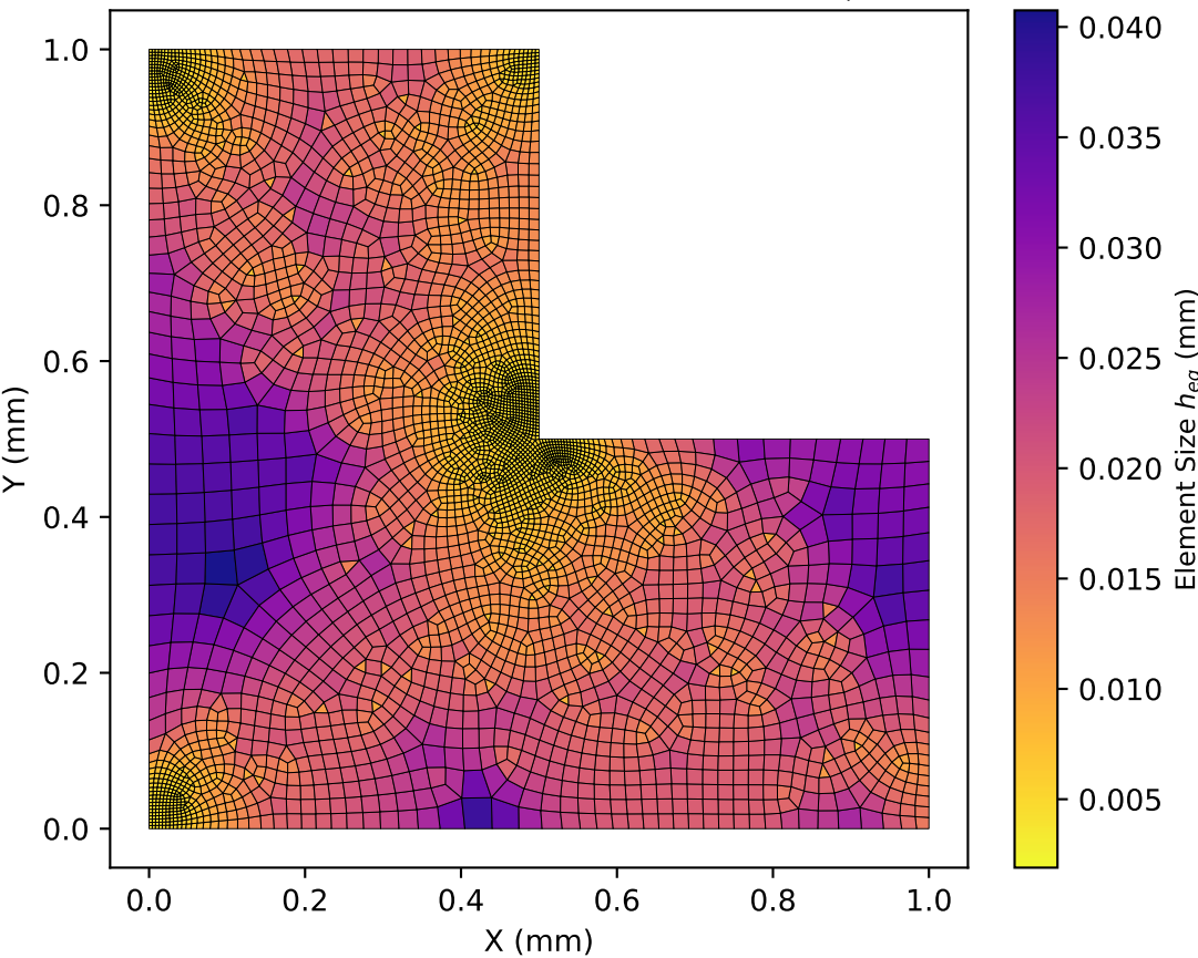
(b) Adapted Mesh (4324 elements) (True Element Edges Shaded by h_{eq} )
