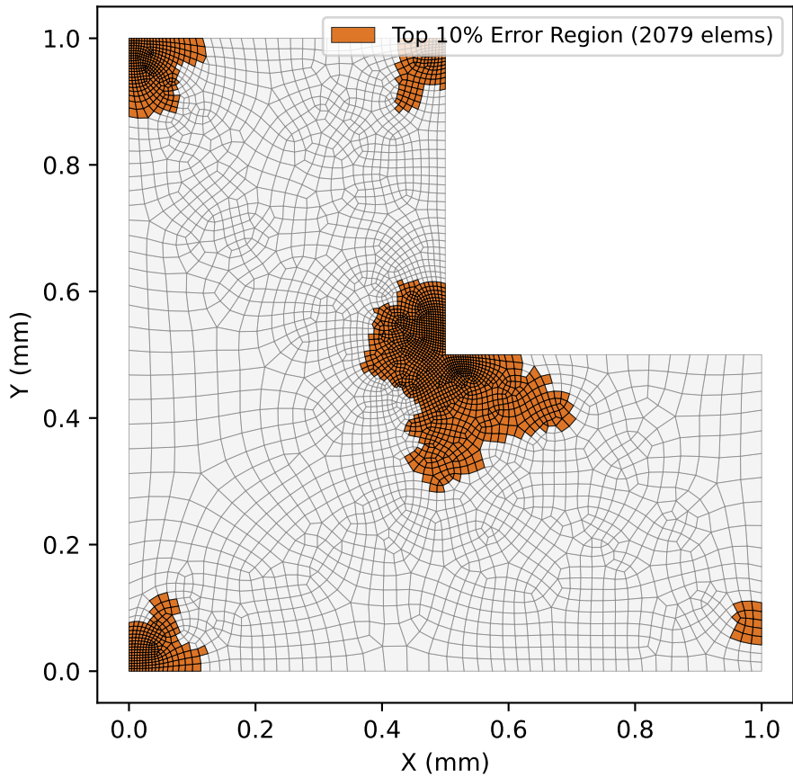
(c) High-Error Singularity Alignment (Top 10% MISESERI Overlaid on Adapted Edges)
