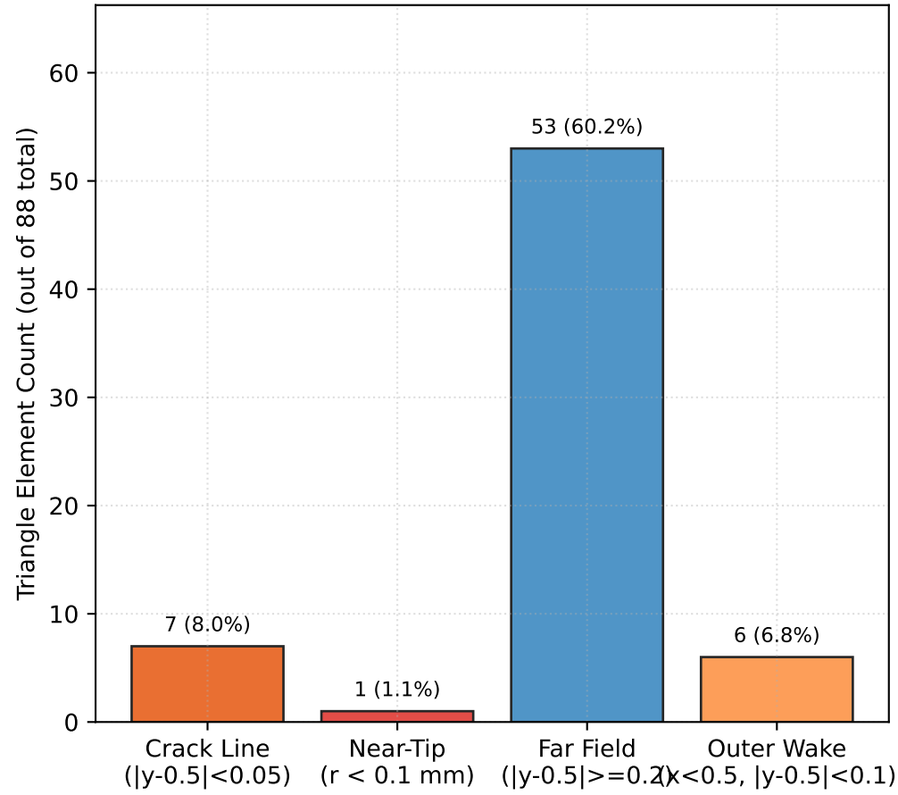
(c) Triangle Spatial Localization Breakdown
