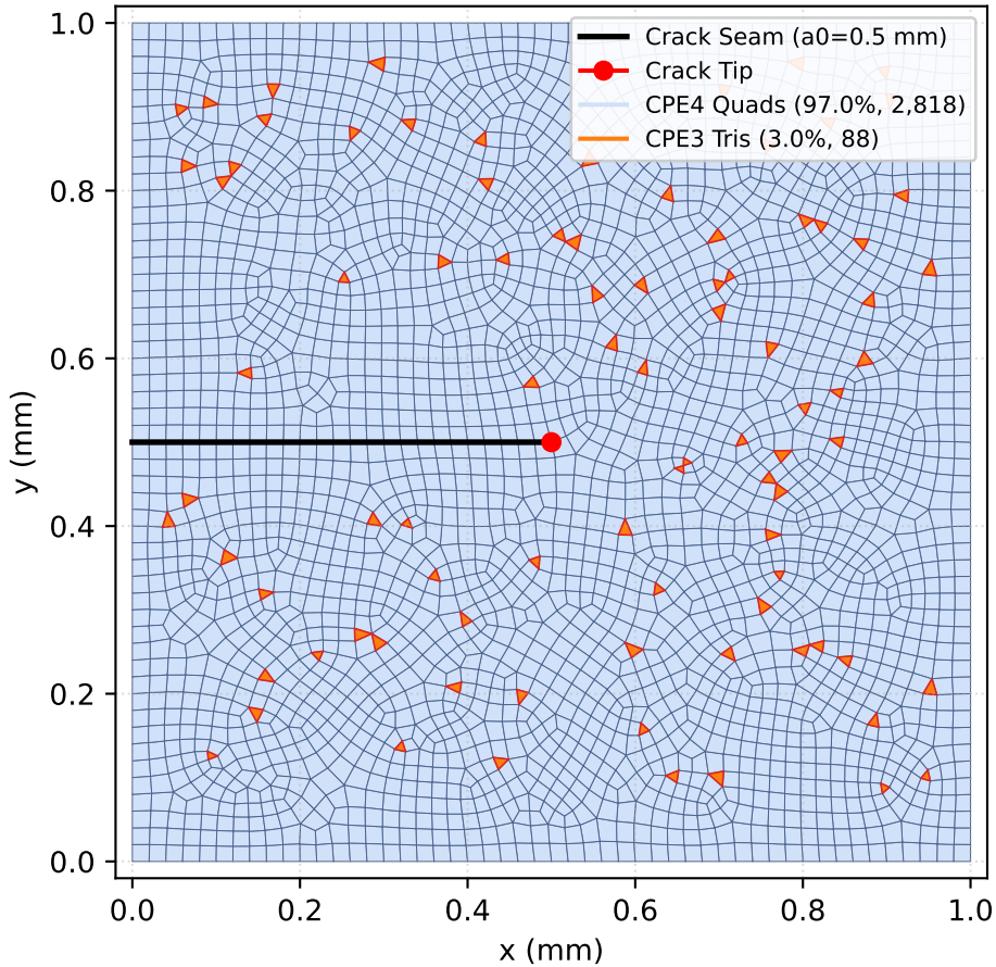
(a) 2,906 Project Coarse Mesh Topology
