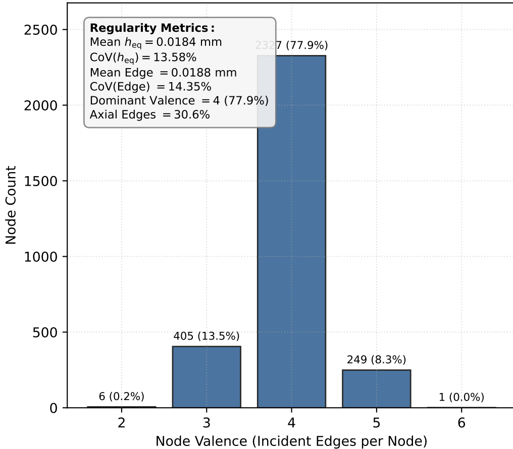
(b) Node Valence & Edge Length Regularity
