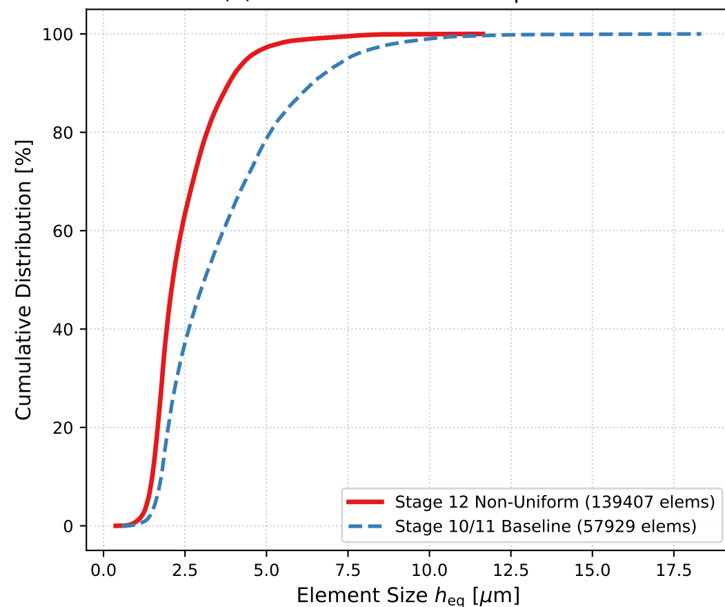
(b) Element Size CDF Comparison
