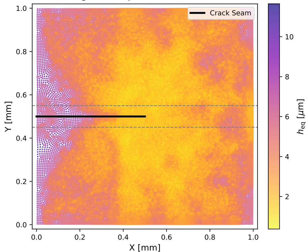
(a) Stage 12 Adapted Mesh ( N = 139407 )
