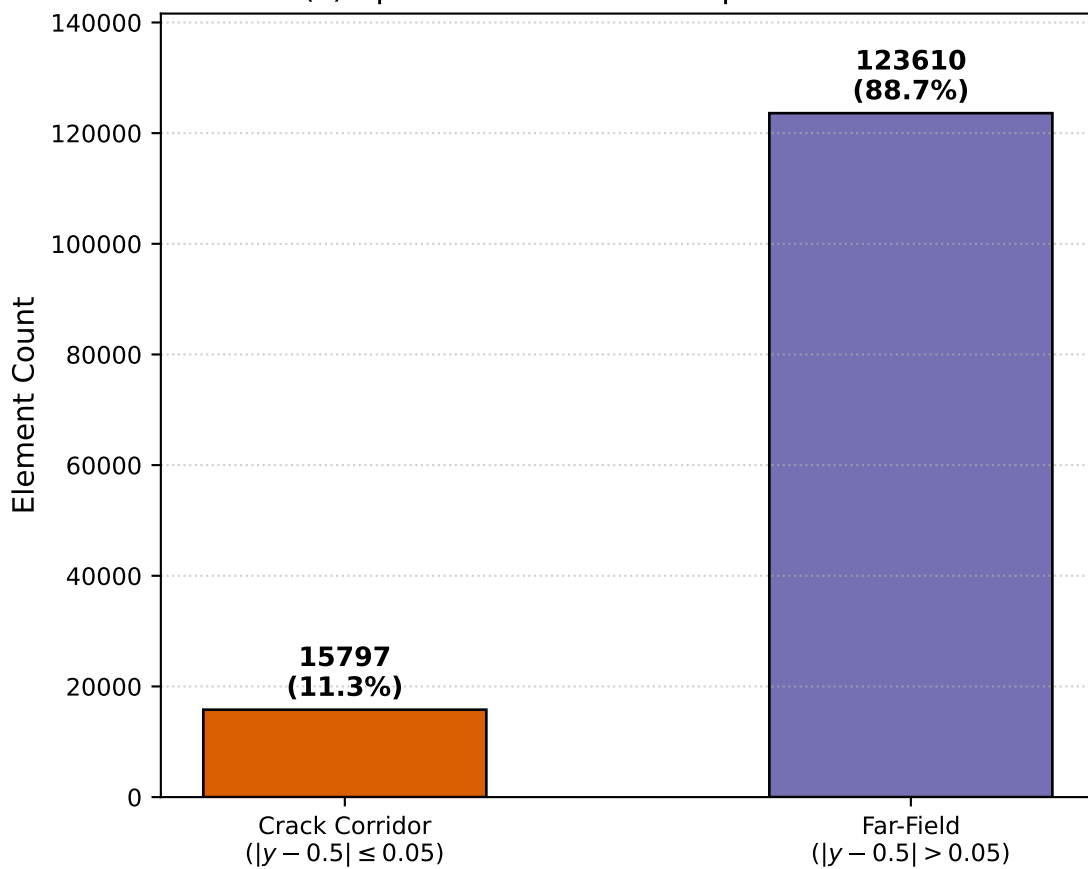
(c) Spatial Partition of Adapted Elements
