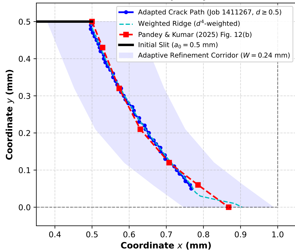
(a) Extracted Crack Trajectory vs. Literature
