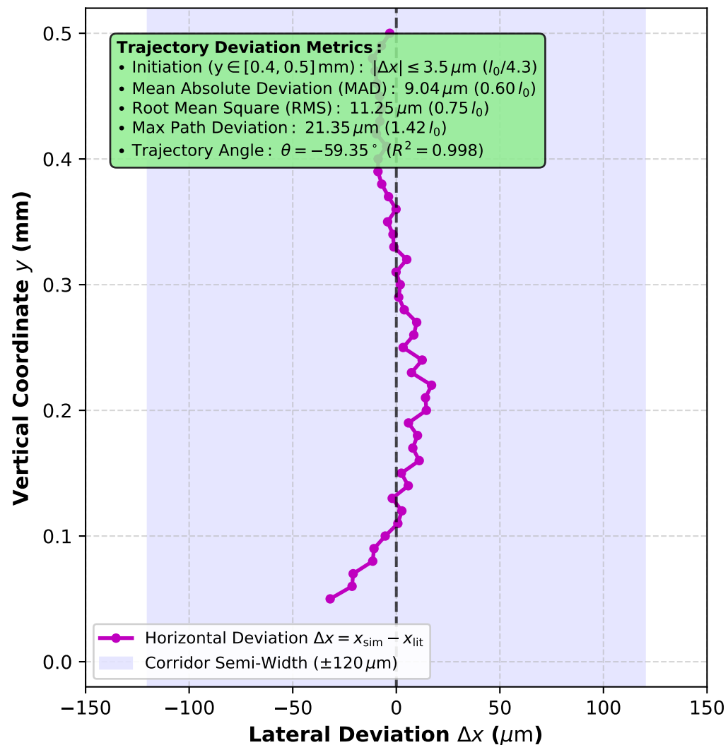
(b) Crack Path Deviation Profile
