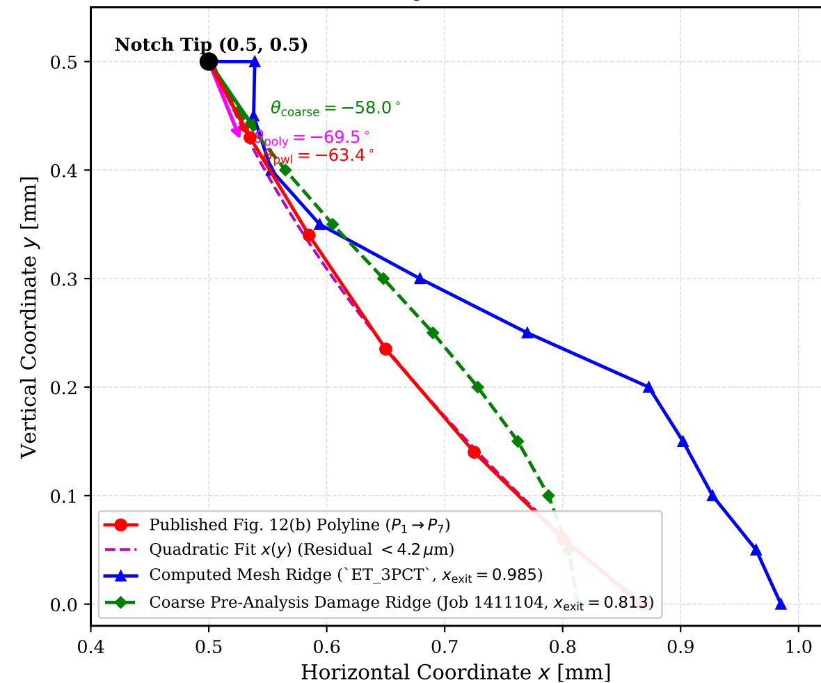
(c) Local Element Resolution along Crack Paths ( l_0 = 15.0 \mu\text{m} )
