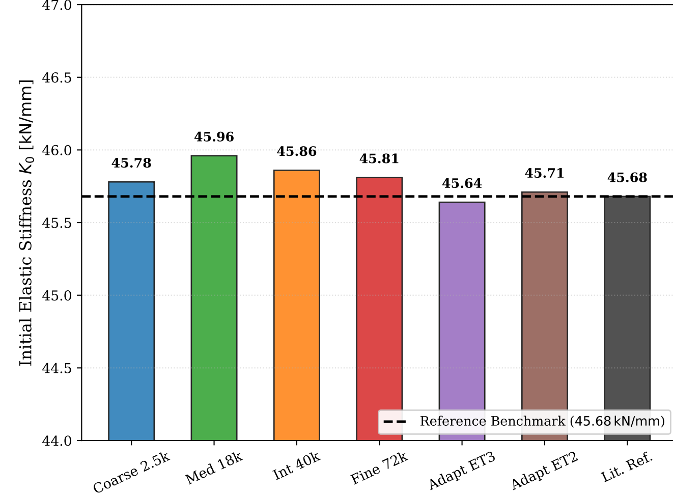
(c) Initial Elastic Stiffness Invariance ( < 0.65\% Spread)
