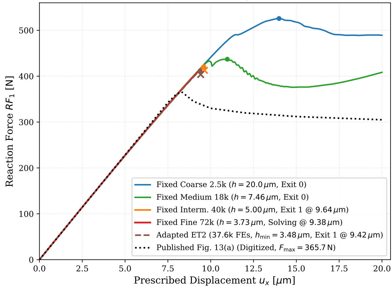
(a) Global Mode-II Shear Response ( RF_1 vs. u_x )
