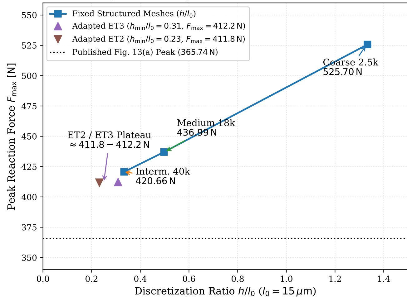
(b) Spatial Convergence of Peak Load ( F_{\max} vs. h/l_0 )
