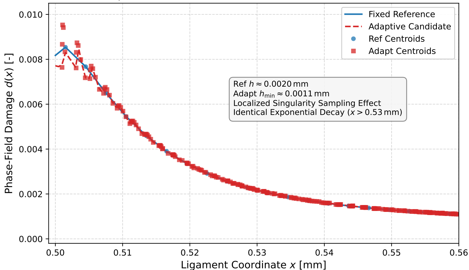
Crack-Tip Localization Zoom ( x \in [0.50, 0.56] mm, u = 0.0010 mm)
