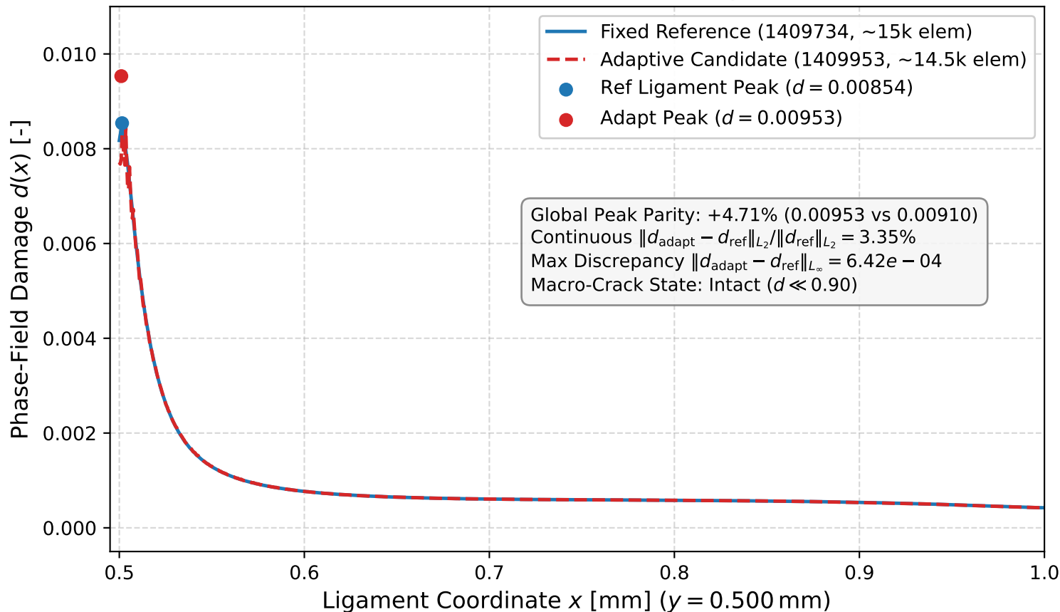
Mode-I Ligament Phase-Field Profile Overlay ( u = 0.0010 mm)
