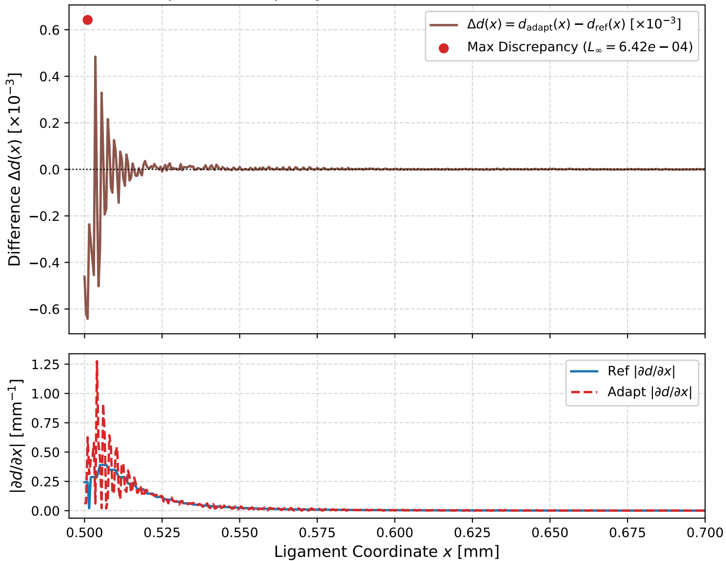
Spatial Discrepancy & Gradient Audit ( u = 0.0010 mm)
