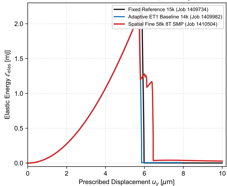
(c) Stored Elastic Strain Energy \mathcal{E}_{\text{elas}}(u_y)
