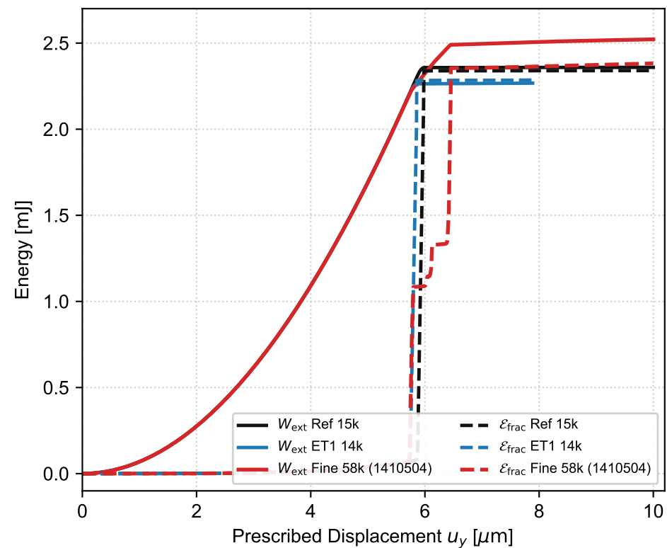
(b) External Work W_{\text{ext}} & Fracture Surface Functional \mathcal{E}_{\text{frac}}
