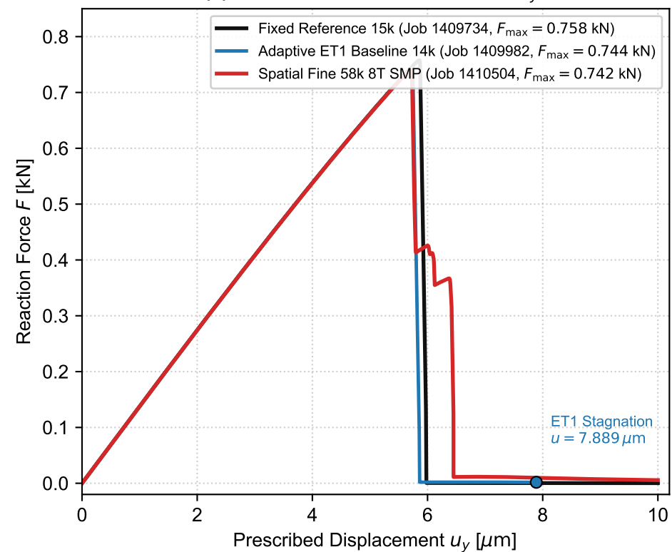
(a) Structural Reaction Force F(u_y)
