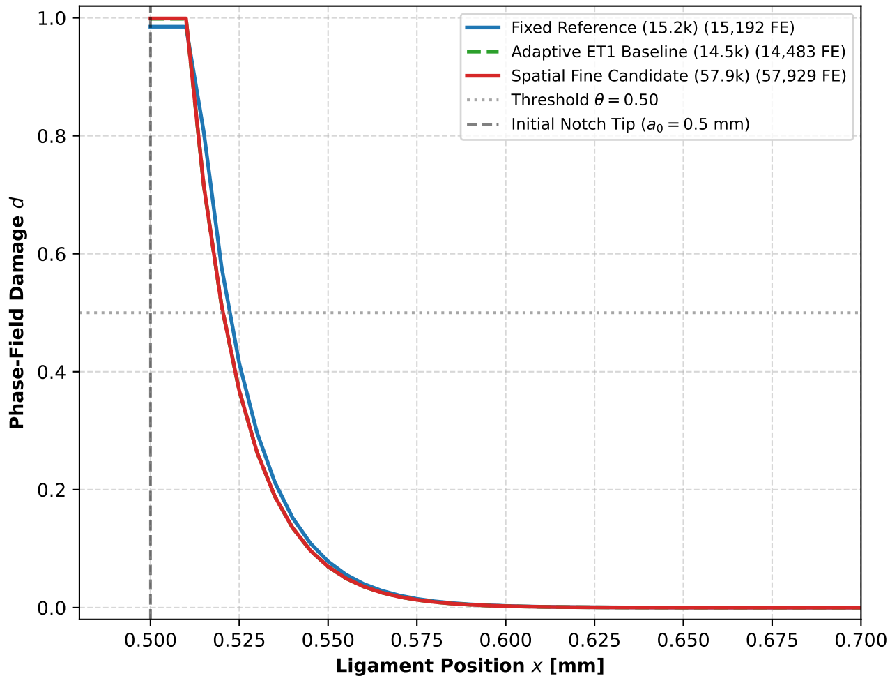
(a) Ligament Damage d(x, y = 0.5 \text{ mm}) at Peak ( u = 5.717 \mu\text{m} )
