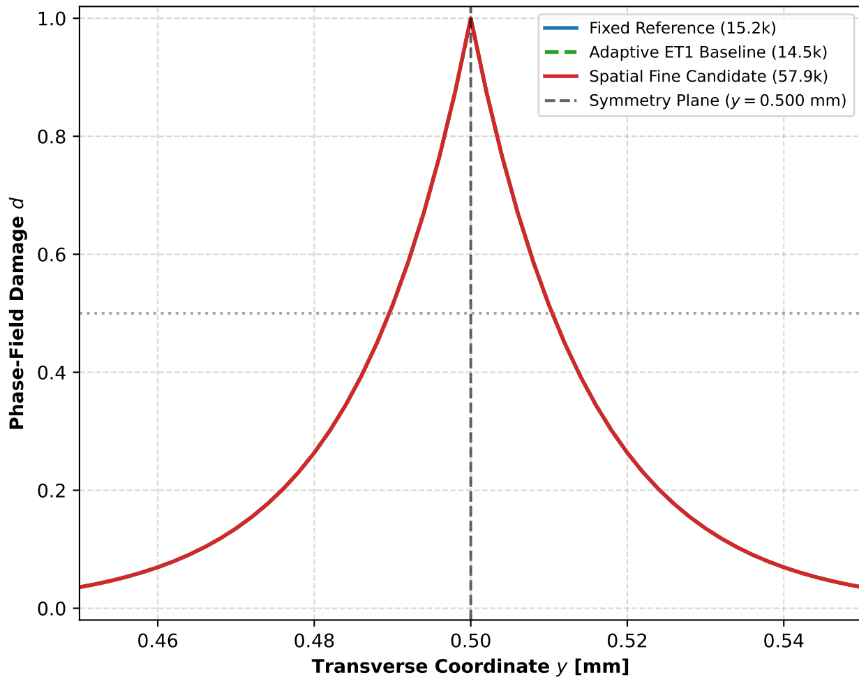
(c) Transverse Damage Profile d(x = 0.55 \text{ mm}, y) ( u = 6.0 \mu\text{m} )
