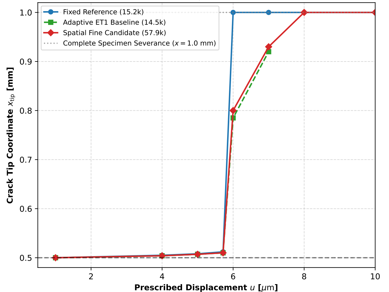
(b) Crack Tip Position x_{\text{tip}}(\theta = 0.5) vs Displacement u
