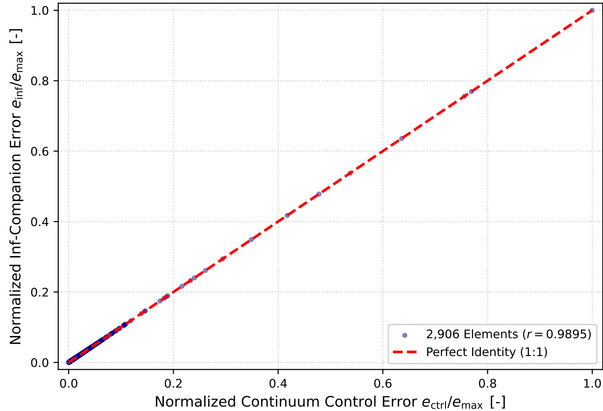
(a) Spatial Invariance & Linear Scaling ( r = 0.9895 )
