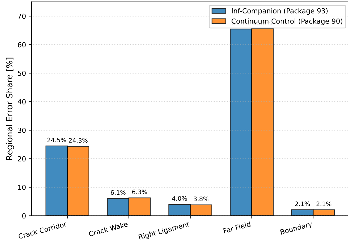
(b) Regional Error Distribution Invariance
