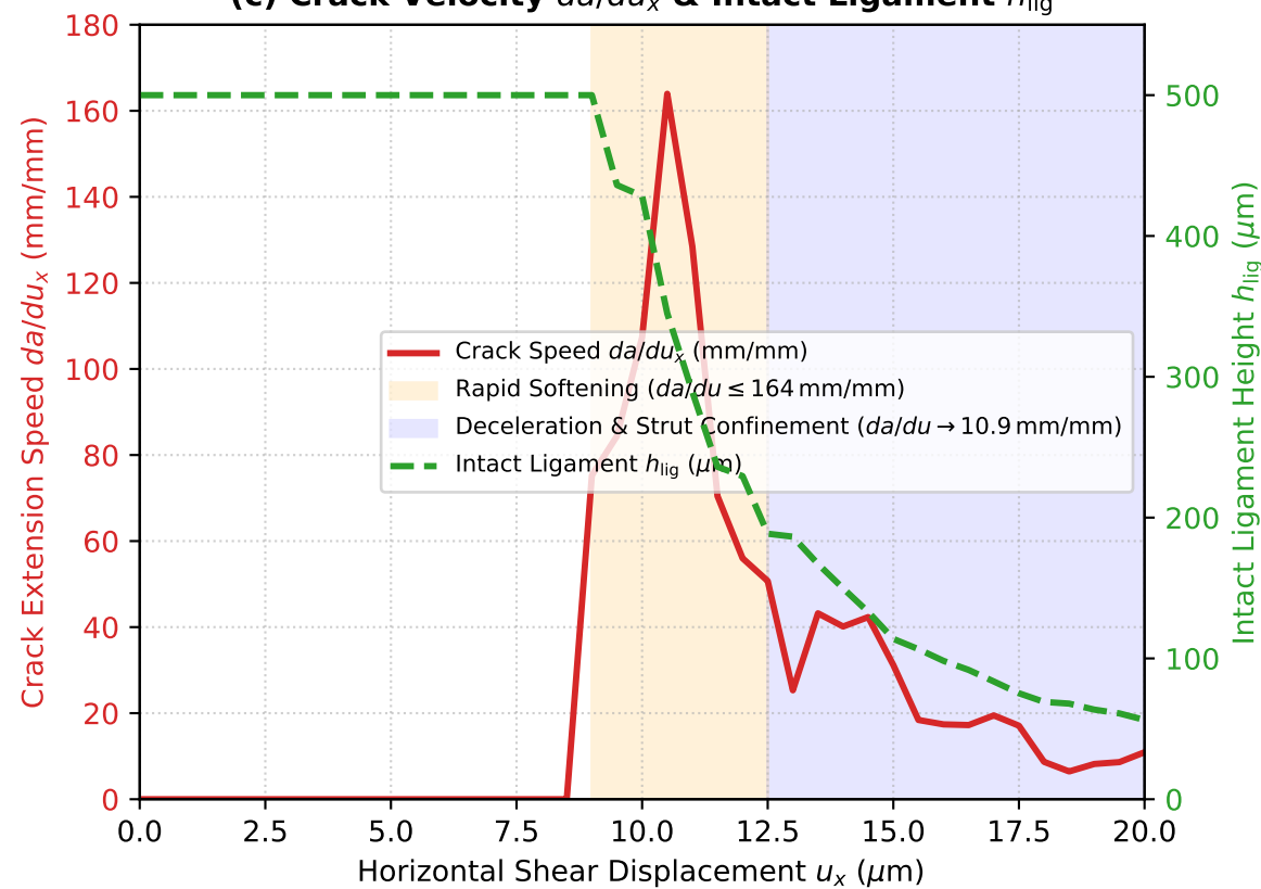
(c) Crack Velocity da/du_x & Intact Ligament h_{\text{lig}}
