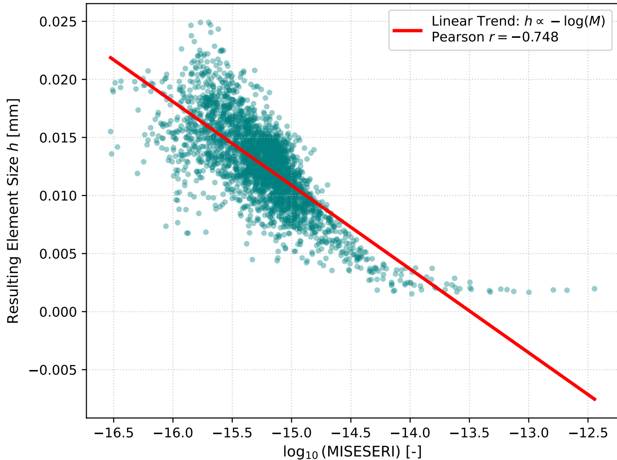
(a) Element Sizing vs Upstream MISES ER I Strict Inverse Correlation Proves Deterministic Remeshing
