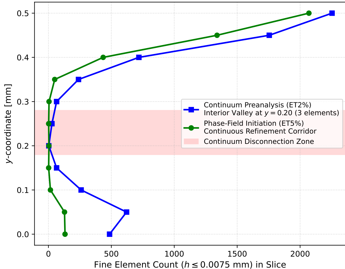
(b) Fine Element Profile along Specimen Height Root Cause of 20% Corridor Disconnection in ET2
