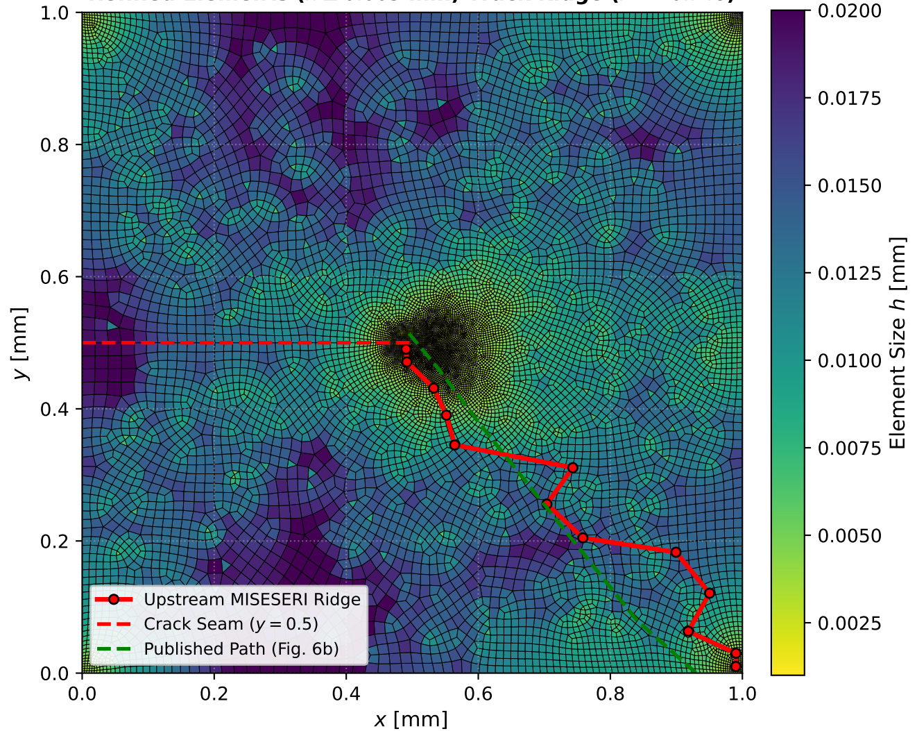
(b) Resulting Native Adaptive Mesh (11,972 Elements)
