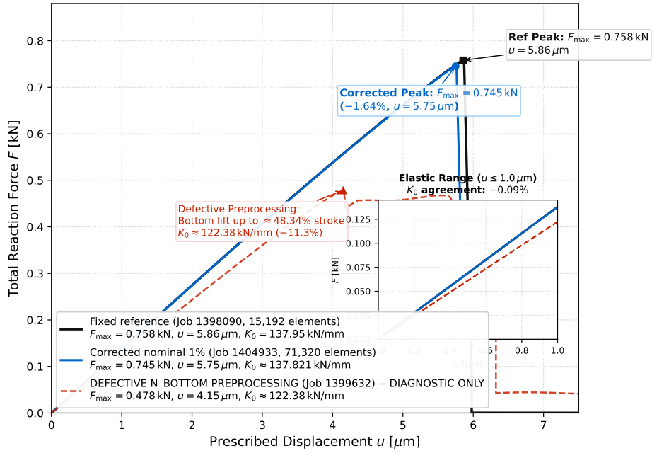
Figure 2.7: Force–displacement response demonstrating reference-consistent structural stiffness recovery (within 0.09%) upon correcting the N_BOTTOM card format.
