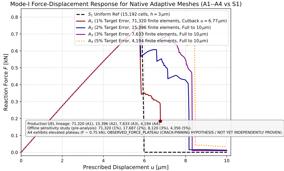
Figure 6.7: Force-displacement curves for native adaptive cases ( A_1 – A_4 ) alongside baseline S_1 .
