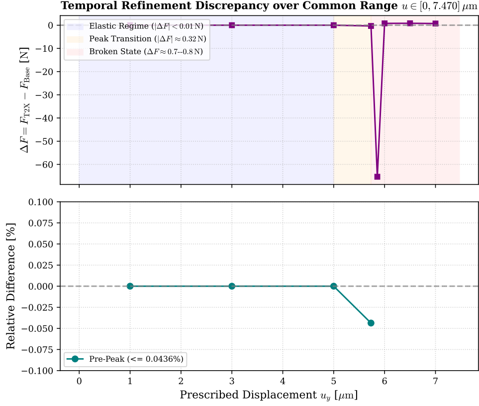
Figure 6.5: Pointwise reaction force discrepancy \Delta F = F_{2\times} - F_{\text{base}} and relative error |\Delta F|/F , confirming sub-0.044% discrepancy throughout the pre-peak regime.
