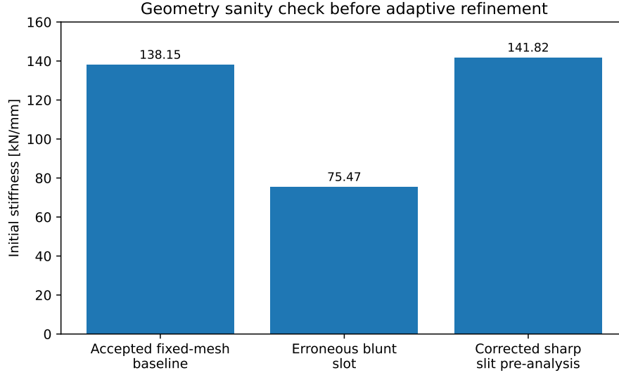
Figure 1.2: Early geometry-sanity-check comparison of structural stiffness K_0 : uncracked solid ( \approx 138.15 kN/mm), blunt notch introducing artificial compliance ( \approx 75.47 kN/mm), and early sharp seam diagnostic ( \approx 141.82 kN/mm). The final governed canonical S_1 sharp-seam reference stiffness is K_0 = 137.945520 kN/mm (Section 1.10).
