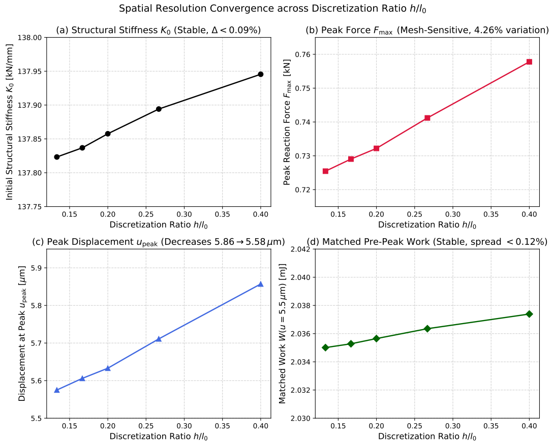
Figure 6.2: Discretization ratio ( h/l_0 ) scaling metrics: (a) initial stiffness K_0 invariance; (b) peak reaction force F_{\max} ; (c) peak displacement u_{\text{peak}} ; (d) matched-displacement external work W_{\text{trap}} at u = 5.50 \mu\text{m} .
