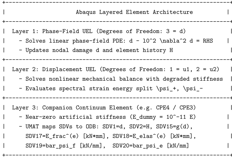
Figure 1.1: Schematic representation of the layered user-element (UEL/UMAT) architecture in Abaqus.
