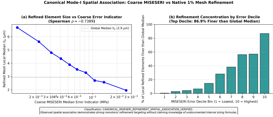
Figure 2.5: Empirical spatial association between coarse MISESeri and adapted element size h for the Mode-I benchmark.
