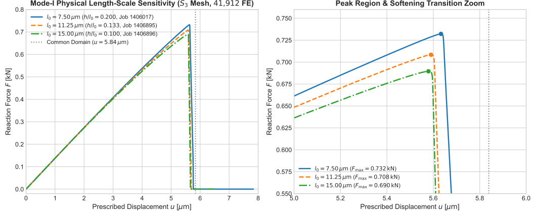
Figure 6.8: Mode-I clean single-variable length-scale ( l_0 ) sensitivity on fixed structured S_3 mesh (41,912 FE): (a) global F – u response highlighting common comparison domain u \in [0, 5.839] \mu\text{m} ; (b) peak-neighborhood zoom illustrating monotonic load reduction and earlier peak displacement with increasing l_0 .
