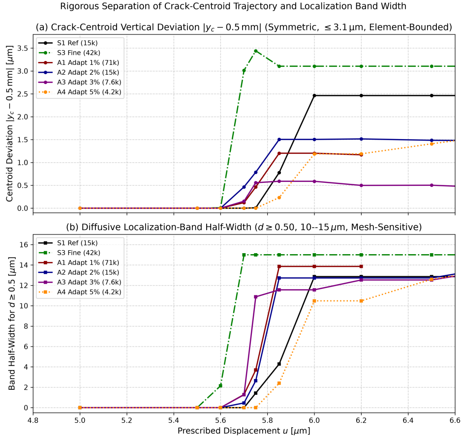
Figure 6.12: Rigorous separation of (a) crack-centroid trajectory ( |y_c - 0.5| \leq 3.1 \mu\text{m} , symmetric) and (b) damage localization-band half-width ( 10\text{--}15 \mu\text{m} , resolution-limited).
