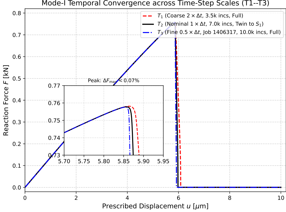
Figure 6.3: Temporal convergence across time increment scales ( T_1 : 2\times , T_2 : 1\times , T_3 : 0.5\times ), demonstrating step-size invariance of the mechanical peak.
