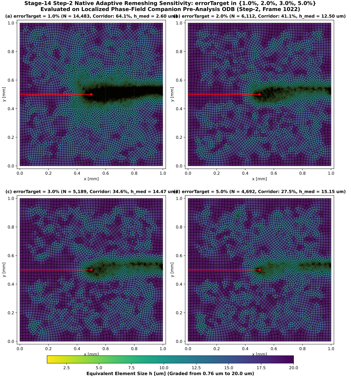
Figure 2.8: Parametric sensitivity of native Abaqus adaptiveRemesh across four error targets ( \text{errorTarget} \in \{1.0\%, 2.0\%, 3.0\%, 5.0\%\} ) evaluated on the localized Stage-14 Step-2 phase-field pre-analysis ODB. Color contours depict equivalent element size h_{\text{eq}} \in [0.76, 20.0] \mu\text{m} . ET1 retains dense, target-like crack-ligament refinement (64.12% corridor share), whereas ET2, ET3, and ET5 progressively under-refine the horizontal propagation path.
