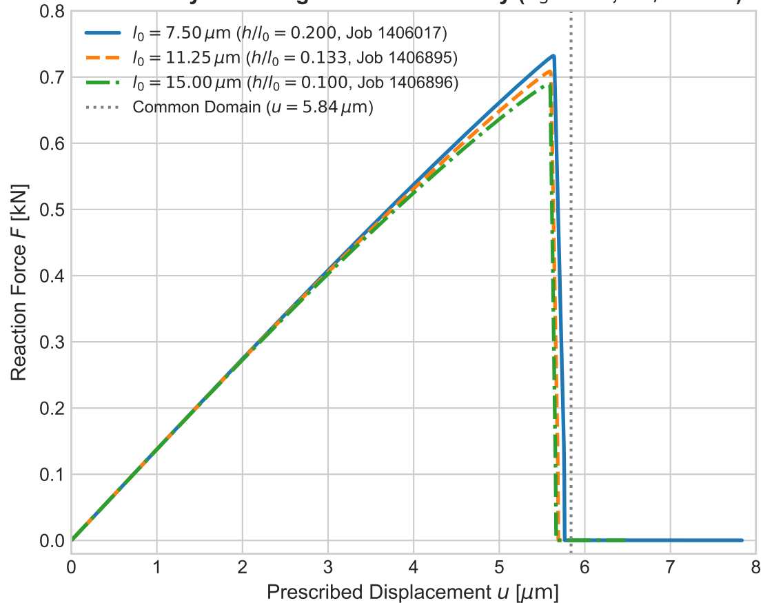
Mode-I Physical Length-Scale Sensitivity ( S_3 Mesh, 41,912 FE)
