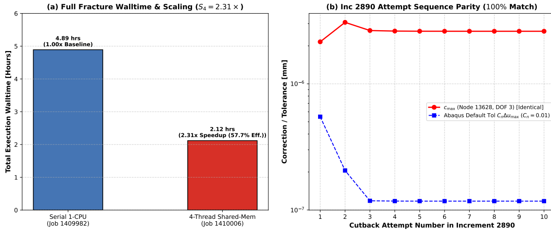
Fig. 4.35.: Stage 14U-AJ scaling and cutback attempt parity: (a) Full fracture execution walltime reduction from 4.89 hrs (Serial) to 2.12 hrs (4-Thread), achieving measured speedup S_4 = 2.31\times and saving 2.77 hrs per solve; (b) Increment 2890 cutback attempt sequence comparing solution correction c_{\max} (red circles, Node 13628, DOF 3) against the shrinking Abaqus tolerance C_n \Delta u_{\max} (blue squares), illustrating 100% bitwise attempt parity between serial and threaded solvers.
