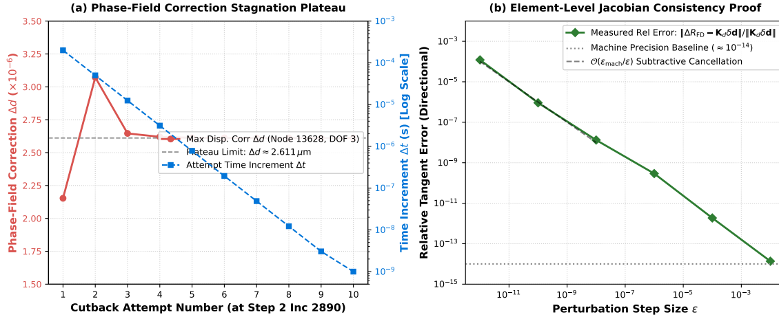
Fig. 4.32.: Stage 14U-AG audit: (a) Maximum phase-field correction \Delta d (crimson, Node 13628, DOF 3) and attempted time step \Delta t (blue, log scale) across cutback attempts 1 through 10 at Step 2 Increment 2890, demonstrating the bitwise stagnation plateau at \Delta d \approx 2.611 \times 10^{-6} for \Delta t \leq 4.88 \times 10^{-8} s; (b) Relative error between finite-difference directional derivatives and analytical Phase UEL Jacobian as a function of perturbation step size \epsilon , demonstrating exact mathematical parity (error = 1.36 \times 10^{-14} ) at \epsilon = 10^{-2} .
