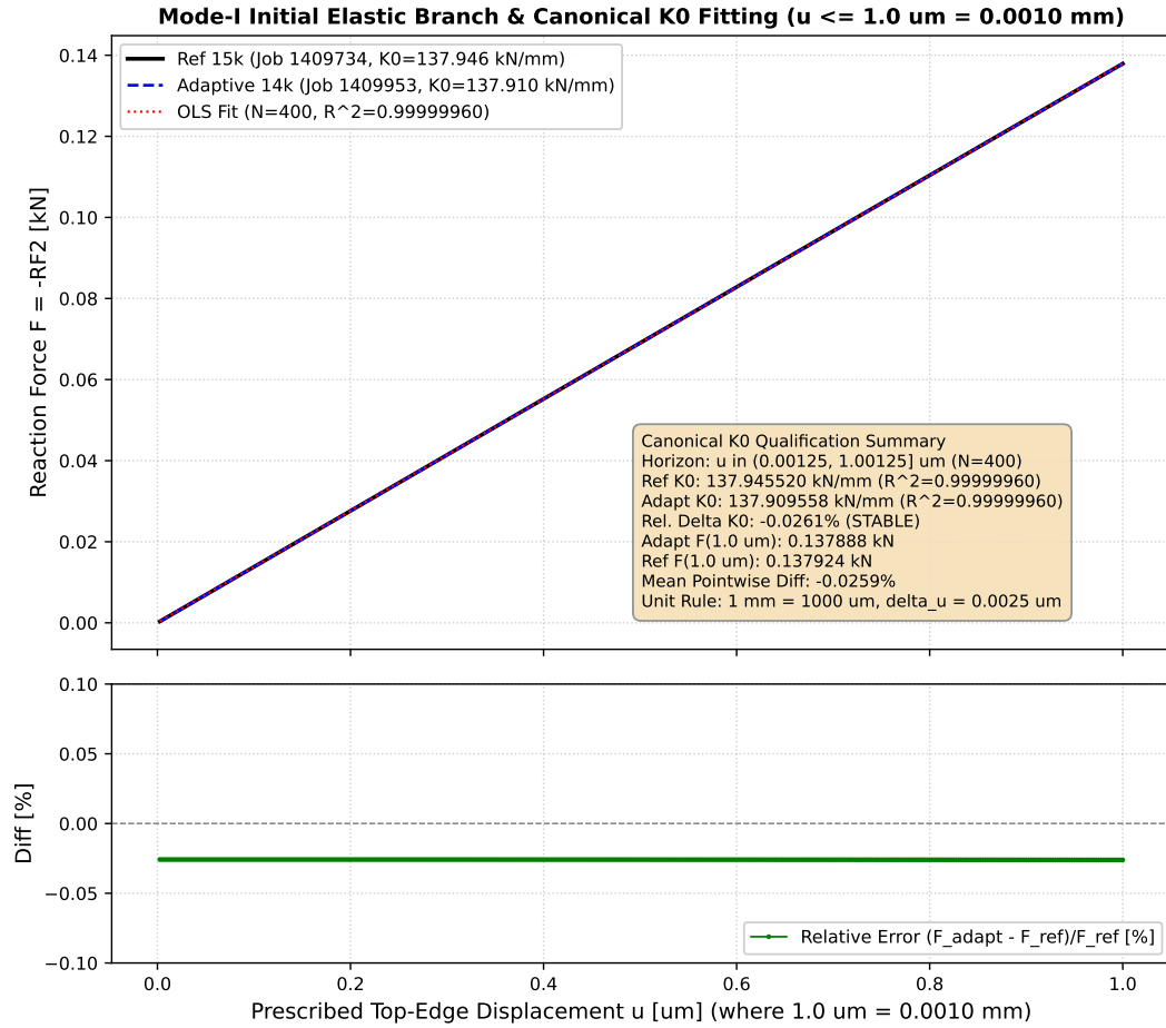
Fig. 4.15.: Canonical structural stiffness ( K_0 ) linear regression across the frozen N = 400 increment window ( u \in (0.00125, 1.00125] \mu\text{m} ). Top: Comparison of reaction force F = -RF_2 between the fixed reference benchmark (Job 1409734) and adaptive solve (Job 1409953) with OLS linear fit. Bottom: Pointwise relative discrepancy (F_{\text{adapt}} - F_{\text{ref}})/F_{\text{ref}} [%] demonstrating sub-0.05% tracking across the entire initial elastic regime.
