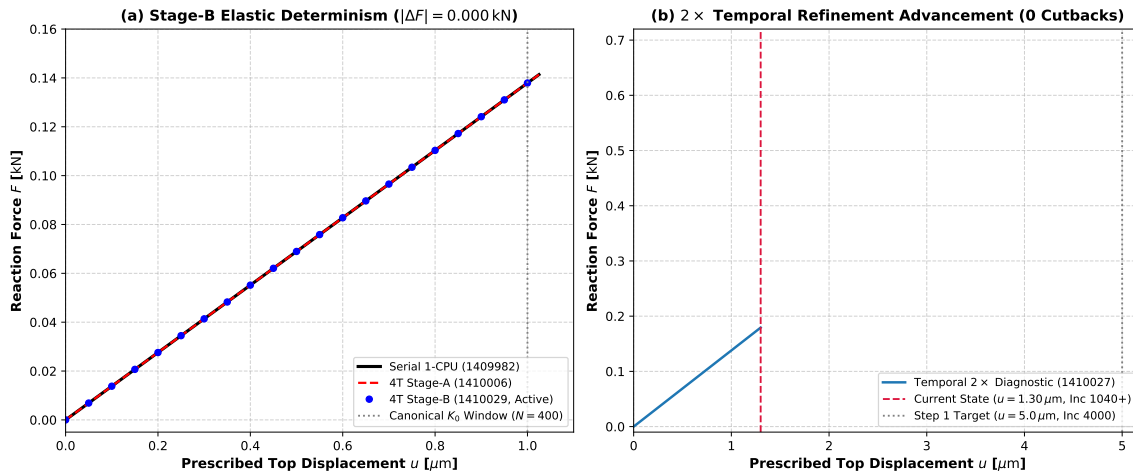
Fig. 4.36.: Stage 14U-AK live execution checkpoint: (a) Initial linear elastic load-displacement response ( F - u ) comparing Serial 1-CPU (black), 4-Thread Stage-A (red dashed), and 4-Thread Stage-B (blue circles), confirming bitwise determinism ( |\Delta F| = 0.000 kN) and canonical stiffness invariance ( K_0 = 137.909558 kN/mm); (b) 2\times temporal refinement diagnostic advancement (Job 1410027) through Step 1 Increment 1040+ ( u = 1.30 \mu\text{m} ) with zero cutbacks.
