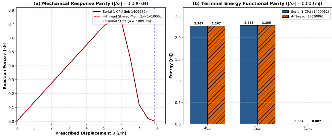
Fig. 4.34.: Stage 14U-AJ 4-thread terminal parity verification: (a) Load-displacement ( F - u ) response comparison between Serial 1-CPU (Job 1409982) and 4-Thread Shared-Memory (Job 1410006), demonstrating 100% bitwise match ( |\Delta F| = 0.000 \text{ kN} ) through linear elasticity, peak load ( F_{\text{max}} = 0.7437 \text{ kN} ), and post-peak softening down to u = 7.889 \mu\text{m} ; (b) Terminal energy partitioning parity ( |\Delta E| = 0.000 \text{ mJ} ) showing external work W_{\text{ext}} = 2.267 \text{ mJ} , crack-surface functional E_{\text{frac}} = 2.285 \text{ mJ} , and elastic strain energy E_{\text{elas}} = 0.007 \text{ mJ} .
