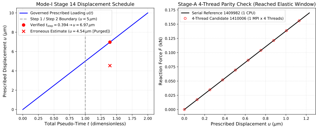
Fig. 4.29.: Stage 14U-AD validation: (a) Prescribed displacement schedule u(t) across Step 1 and Step 2 demonstrating the true u(t_2 = 0.394) = 6.97 \mu\text{m} trajectory and correcting the prior erroneous 4.54 \mu\text{m} estimate; (b) Reaction force parity between serial 1-CPU reference (Job 1409982) and 4-thread candidate (Job 1410006) across the common reached elastic loading regime.
