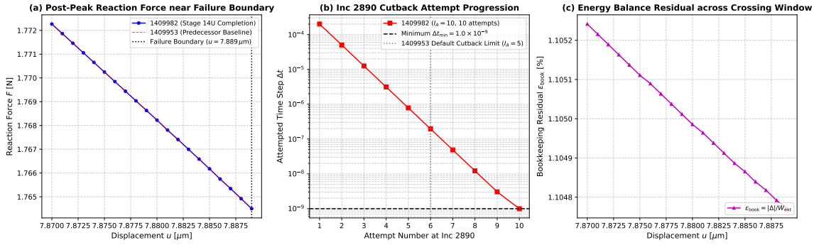
Fig. 4.31.: Stage 14U-AF crossing audit: (a) Reaction force F(u) overlay between predecessor Job 1409953 and completion Job 1409982 in the post-peak softening tail, confirming identical physical equilibrium down to 1.76 N (99.76% load drop); (b) Increment 2890 cutback attempt progression, demonstrating that Job 1409982 actively exercised the extended allowance ( I_A = 10 ) across 10 successive attempts down to the solver floor \Delta t_{\min} = 1.0 \times 10^{-9} compared to predecessor cutback exhaustion at attempt 6; (c) Energy bookkeeping residual \varepsilon_{\text{book}} \approx 1.1048\% across the crossing window.
