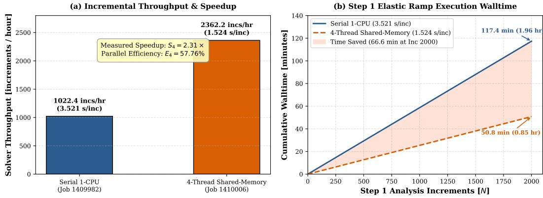
Fig. 4.30.: Stage 14U-AE performance audit: (a) Solver throughput and walltime per increment comparing serial 1-CPU reference (3.521 s/inc, 1,022.4 incs/hr) and 4-thread shared-memory candidate (1.524 s/inc, 2,362.2 incs/hr), demonstrating a measured speedup of S_4 = 2.31\times ( E_4 = 57.76\% ); (b) Cumulative elapsed walltime progression across the 2,000 increments of Step 1, showing a reduction from 117.4 min to 50.8 min (66.6 min saved).
