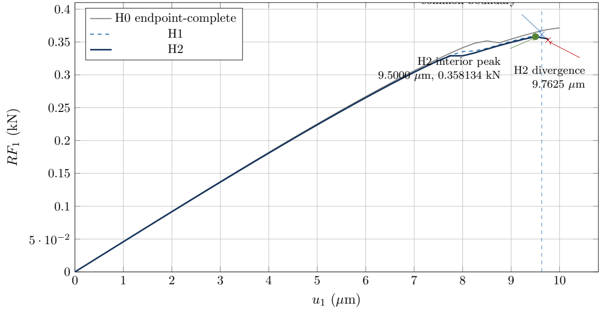
Figure 1. RF_1 – u_1 comparison from primary extracted curves. H2 reproduces the previous solution exactly to 9.25 \mu\text{m} , reaches an interior peak at 9.50 \mu\text{m} , and diverges at 9.7625 \mu\text{m} . H1 diverges at 9.6325 \mu\text{m} ; global H1/H2 peak convergence remains unresolved.
