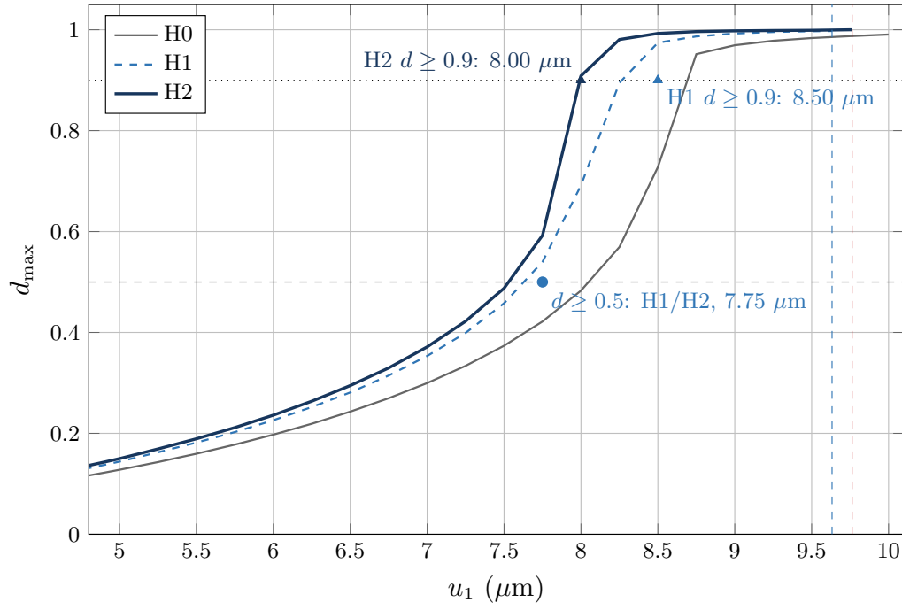
Figure 2. Extended damage evolution. H1 and H2 share d_{\max} \geq 0.5 initiation at 7.75 \mu\text{m} . The d_{\max} \geq 0.9 threshold occurs at 8.00 \mu\text{m} for H2 and 8.50 \mu\text{m} for H1.
