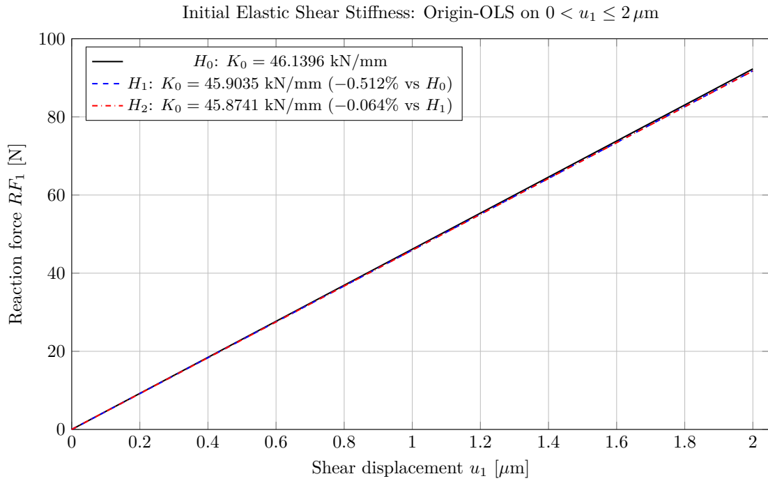
Figure 3. Identical origin-OLS stiffness fits over 0 < u_1 \leq 0.002 mm. K_0 = 46.1396 , 45.9035 , and 45.8741 kN/mm for H0/H1/H2, respectively.
