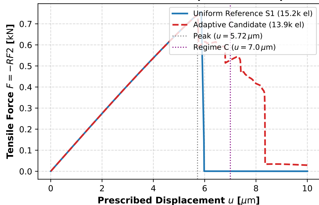
(a) Global Tensile Force-Displacement Response
