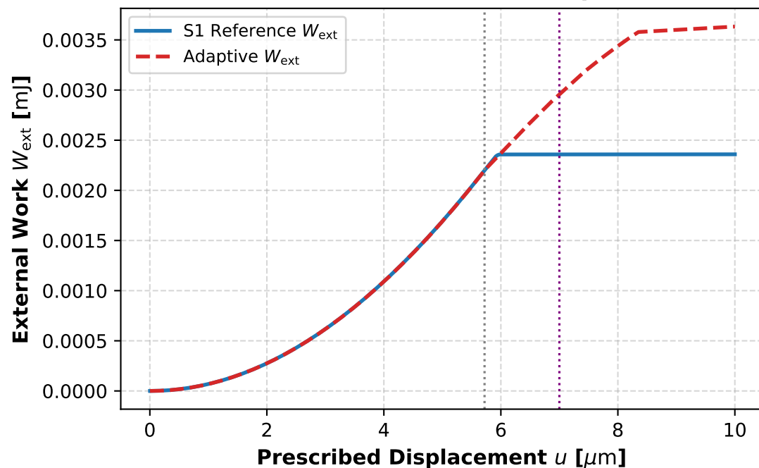
(b) Cumulative External Work Input W_{\text{ext}}(u)
