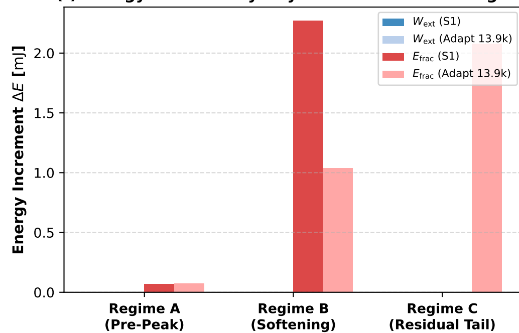
(f) Energy Partition by Physical Deformation Regime
