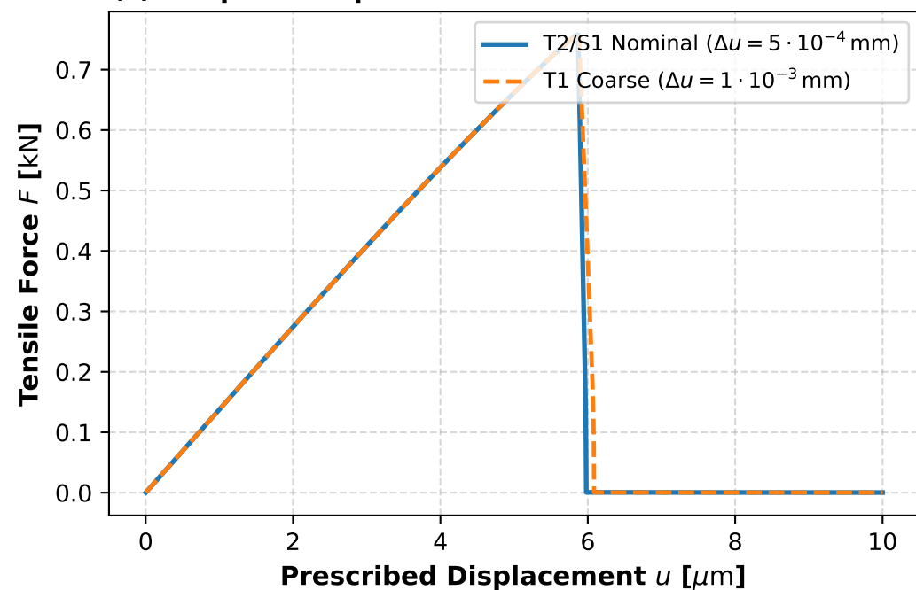
(c) Temporal Step Invariance: T1 Coarse vs T2 Nominal
