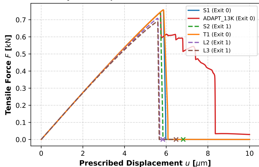
(a) Multi-Family Load-Displacement Curves (Truncations Marked ×)
