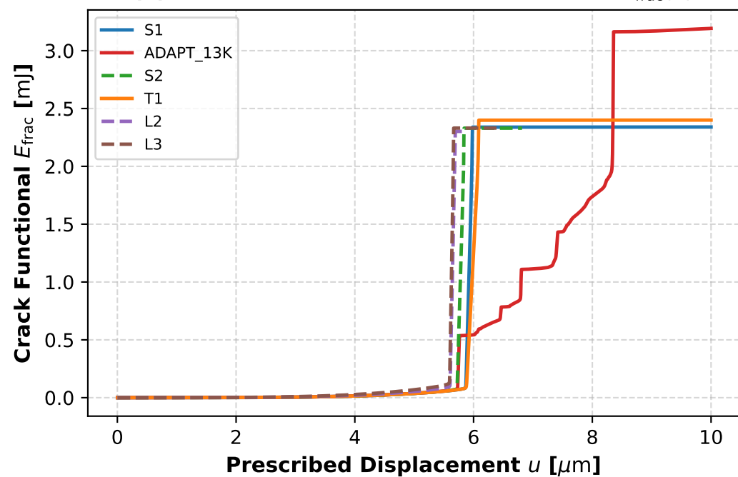
(e) Phase-Field Crack Surface Functional E_{\text{frac}}(u)
