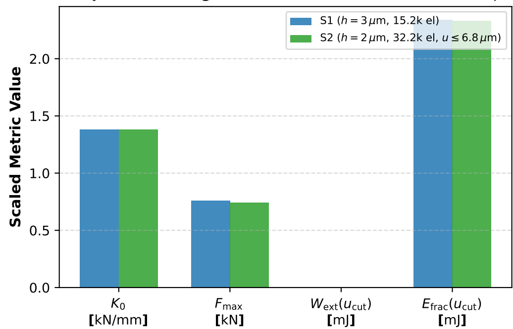
(b) Spatial Convergence: S1 vs S2 at Matched u = 6.82 \mu\text{m}
