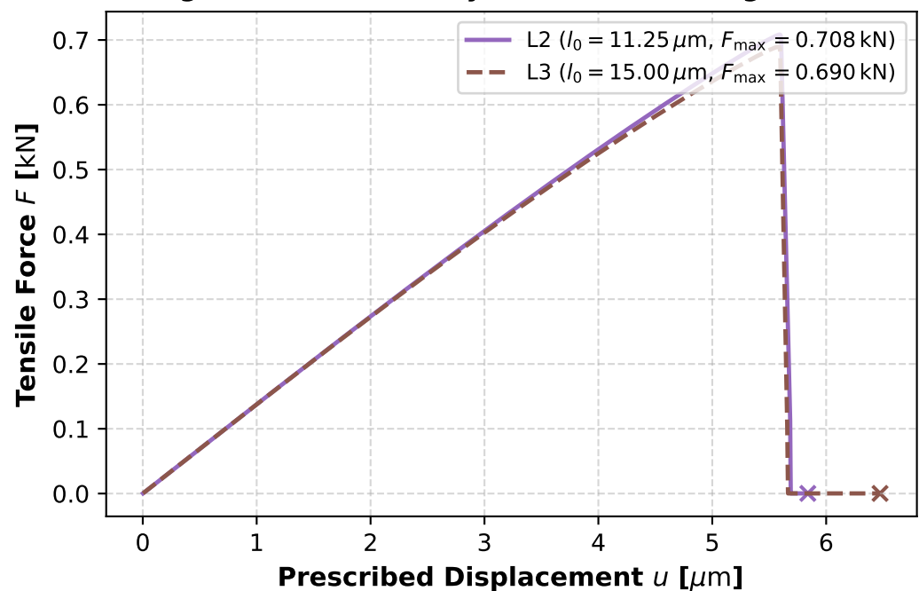
(d) Length-Scale Sensitivity: Peak Load vs Regularization l_0
