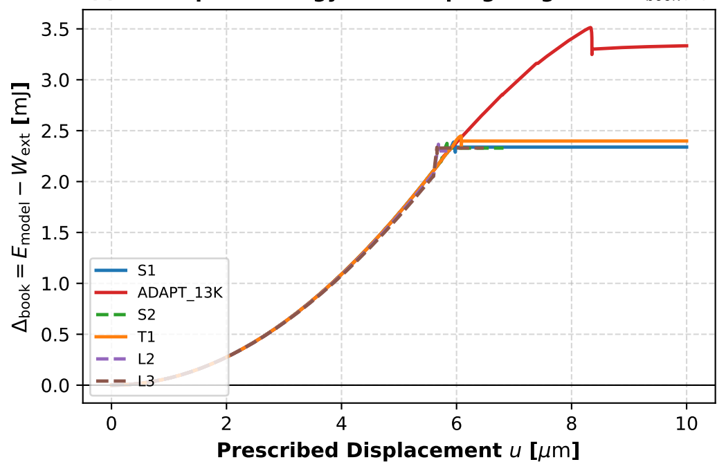
(f) Descriptive Energy Bookkeeping Diagnostic \Delta_{\text{book}}(u)
