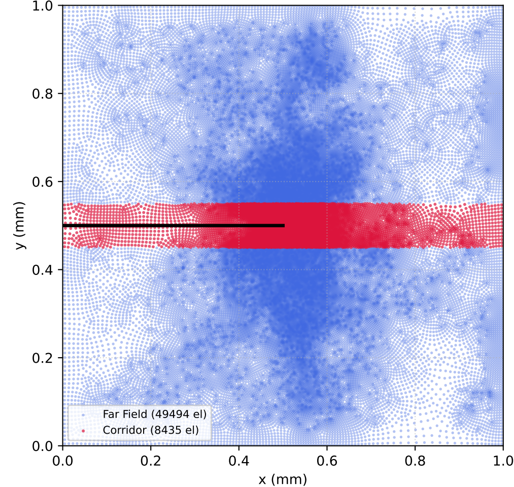
(c) Package 93 Native 1% Mesh 57929 elements (Corridor: 14.6%, Far Field: 85.4%)
