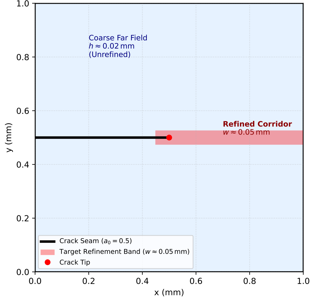
(a) Published Target (Pandey & Kumar 2025 Fig. 6a) 13,941 elements (Narrow Corridor Band)
