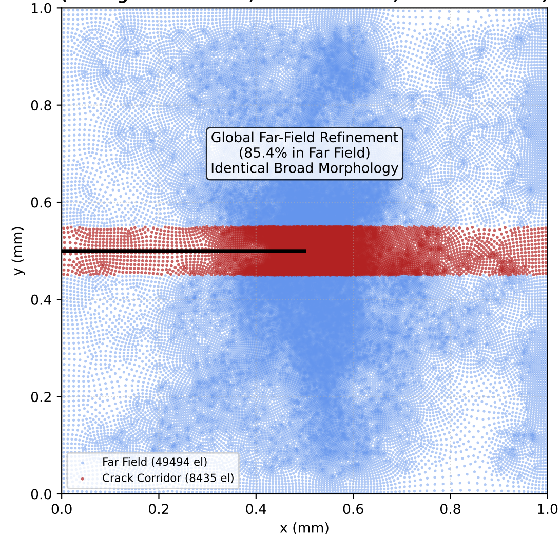
(b) Infinitesimal-Companion Native 1% Mesh (Package 93: 57929 el, Corridor: 14.6%, Far Field: 85.4%)
