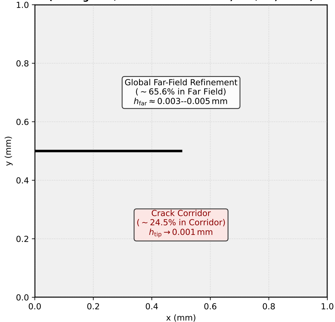
(a) Continuum Pre-Analysis Native 1%% Mesh (Package 90 / Coarse Reference: 71,320 / 48,329 el)
