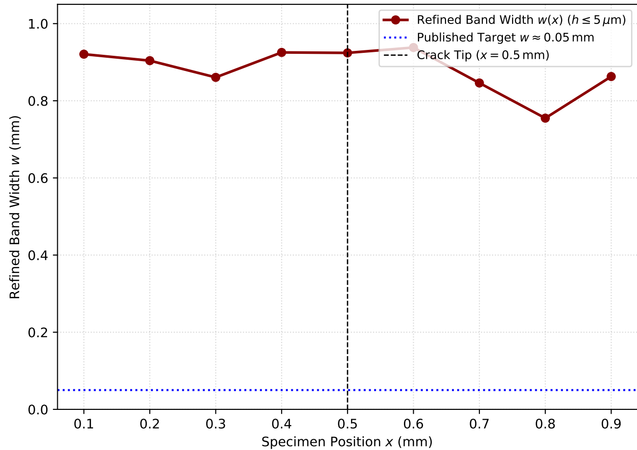
(b) Refinement Bandwidth along Crack Line Observed vs Target Morphology
