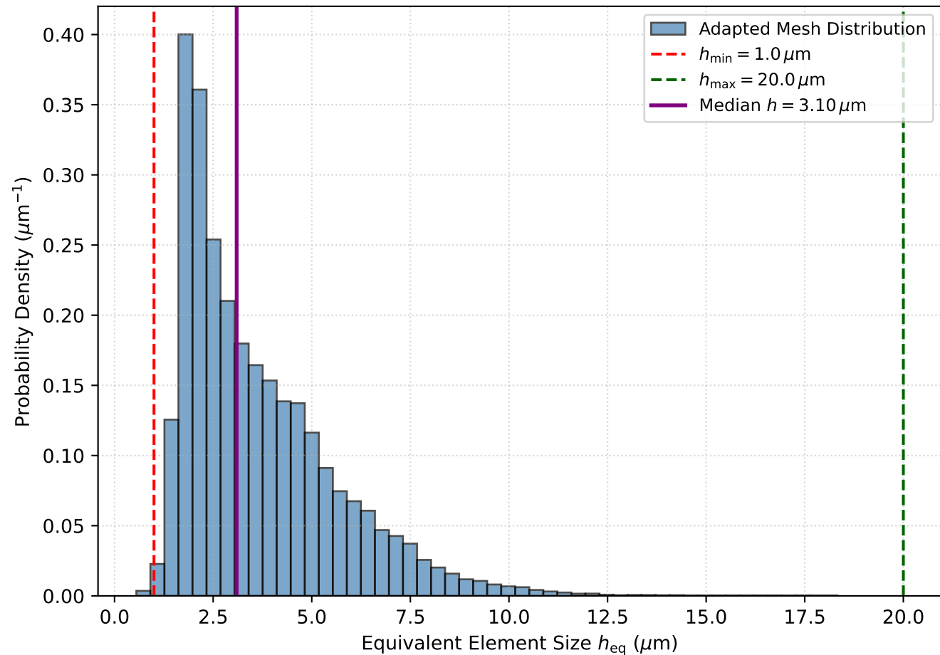
(a) Element Sizing Distribution Bounded within [1.0, 20.0] \mu\text{m}
