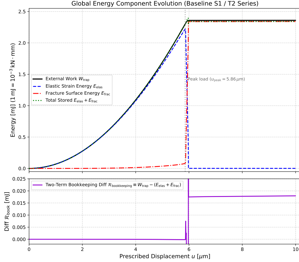
Figure 6.12: Global energy component evolution for the baseline S_1/T_2 trajectory (15,192 elements). The two-term bookkeeping difference remains within \pm 0.008\% over the specifically qualified pre-peak S_1/T_1-T_3 trajectories. In the post-peak regime it reaches +0.7607\% for S_1/T_2 . This quantity is an endpoint bookkeeping difference and is not interpreted as an energy residual or conservation error. GLOBAL_ENERGY_IDENTITY -- NOT_YET_CLOSED.
