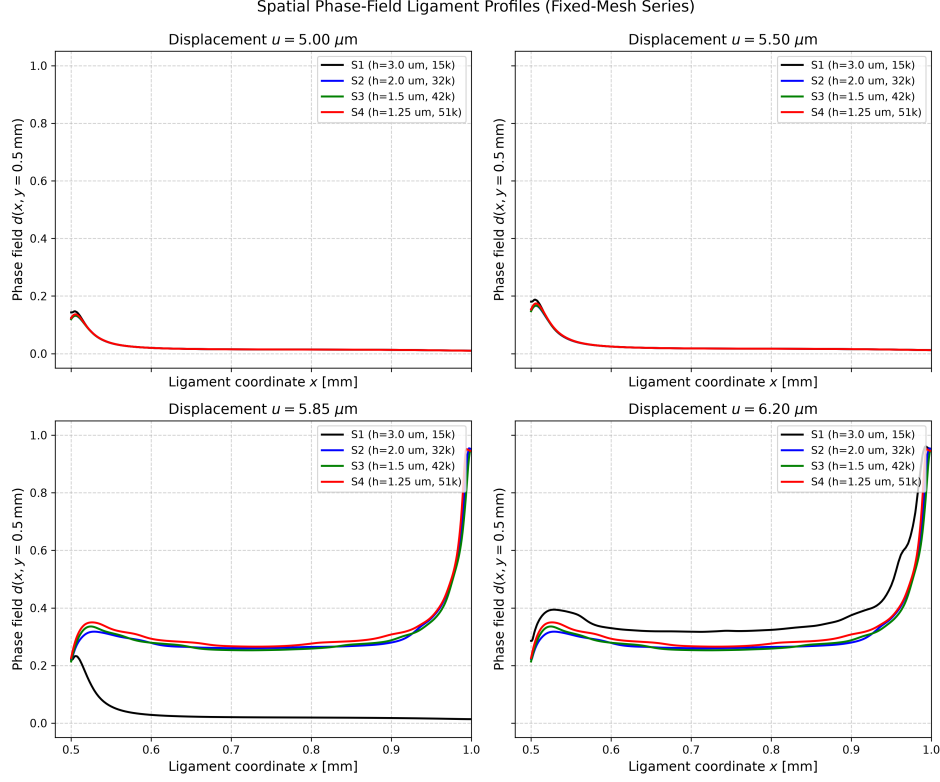
Figure 6.10: Ligament phase-field profiles d(x, y = 0.5 \text{ mm}) for fixed meshes at matched displacement increments.
