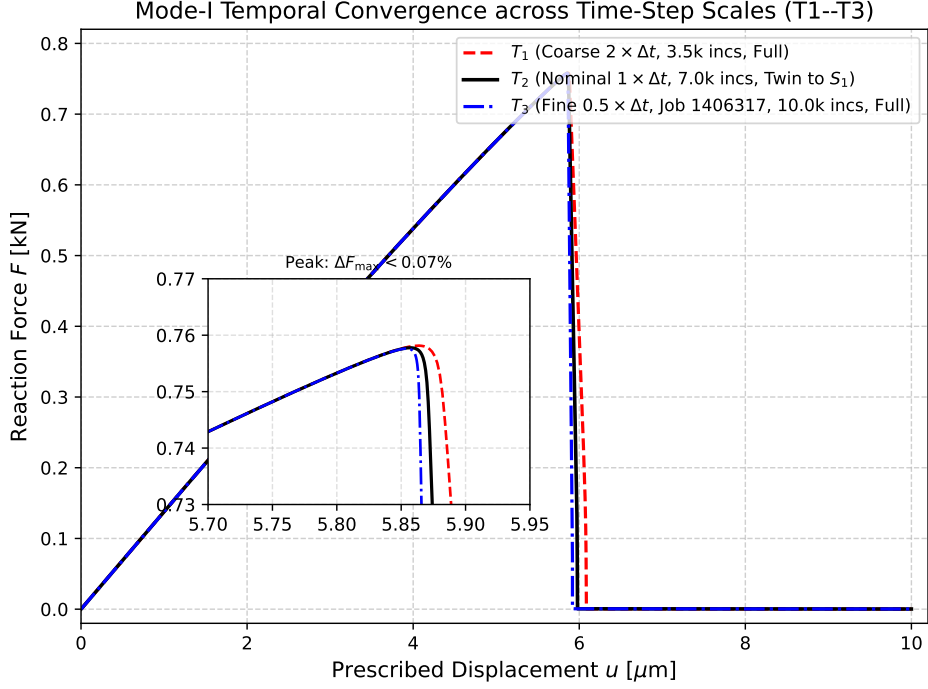
Figure 6.3: Mode-I temporal convergence across time increment scales ( T_1 : 2\times , T_2 : 1\times , T_3 : 0.5\times , Job 1406317.mmmaster02), showing step-size invariance of the mechanical peak.
