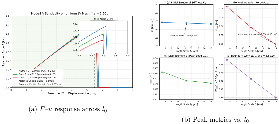
Figure 6.8: Three-point physical length-scale study on fixed S_3 mesh ( h = 1.5 \mu\text{m} ): (a) global force-displacement overlay and (b) variation of K_0 , F_{\max} , u_{\text{peak}} , and matched W_{\text{trap}} at u = 5.50 \mu\text{m} with l_0 .
