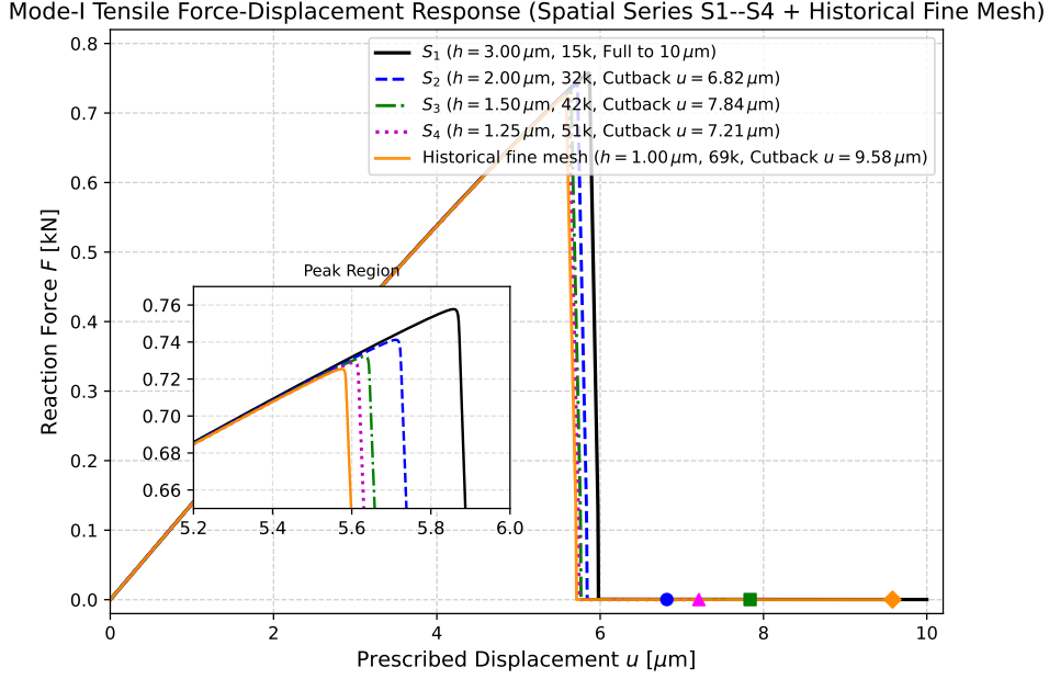
Figure 6.1: Mode-I tensile force-displacement response across uniform mesh resolutions ( S_1 – S_4 plus historical fine mesh), showing closely coincident / stable elastic stiffness and systematic peak load mesh sensitivity.
