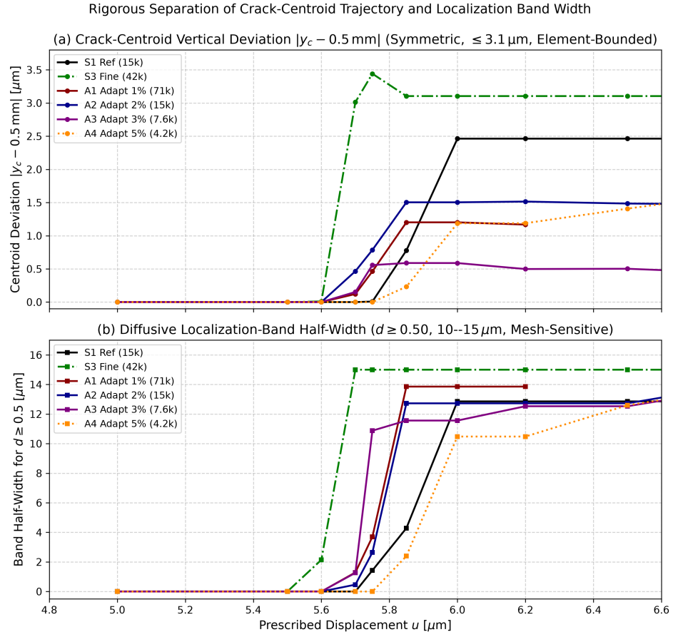
Figure 6.11: Rigorous separation of (a) crack-centroid trajectory ( |y_c - 0.5| \leq 3.1 \mu\text{m} , symmetric) and (b) damage localization-band half-width ( 10\text{--}15 \mu\text{m} , resolution-limited).
