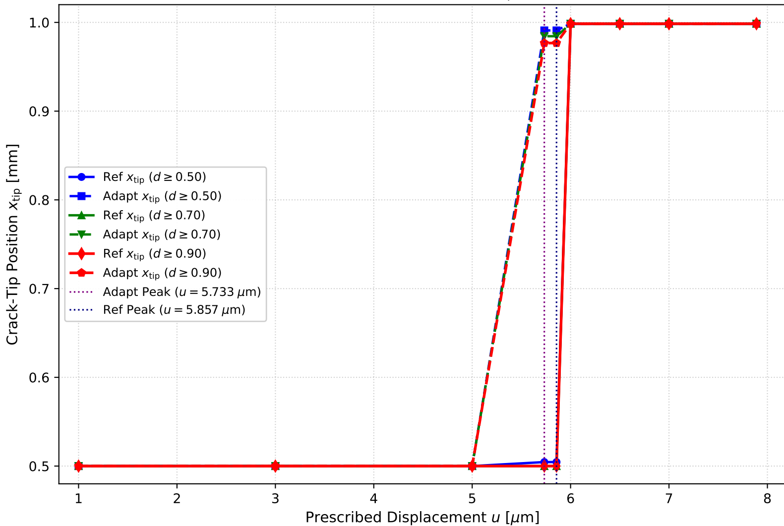
Mode-I Crack-Tip Coordinate Evolution x_{\text{tip}}(u) Across Thresholds
