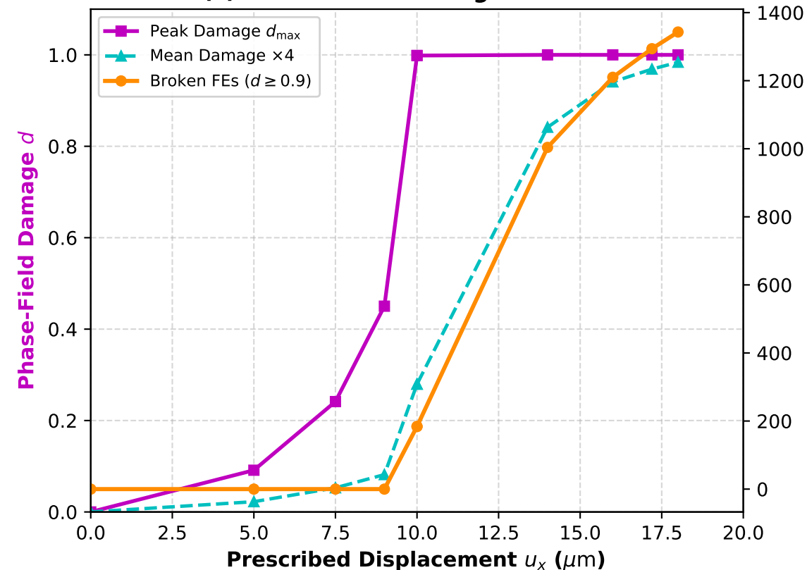
(c) Phase-Field Damage Evolution
