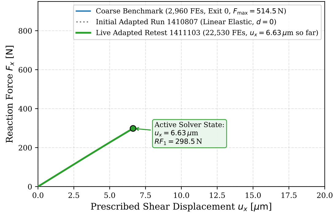
(c) Structural Degradation & Stiffness Softening Trajectory
