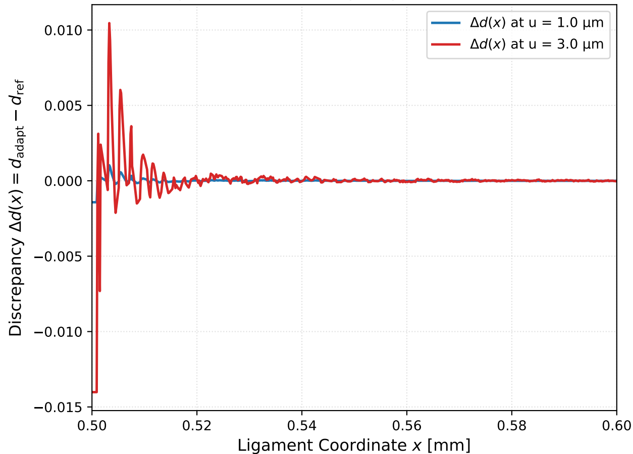
Spatial Profile Discrepancy Evolution \Delta d(x)
