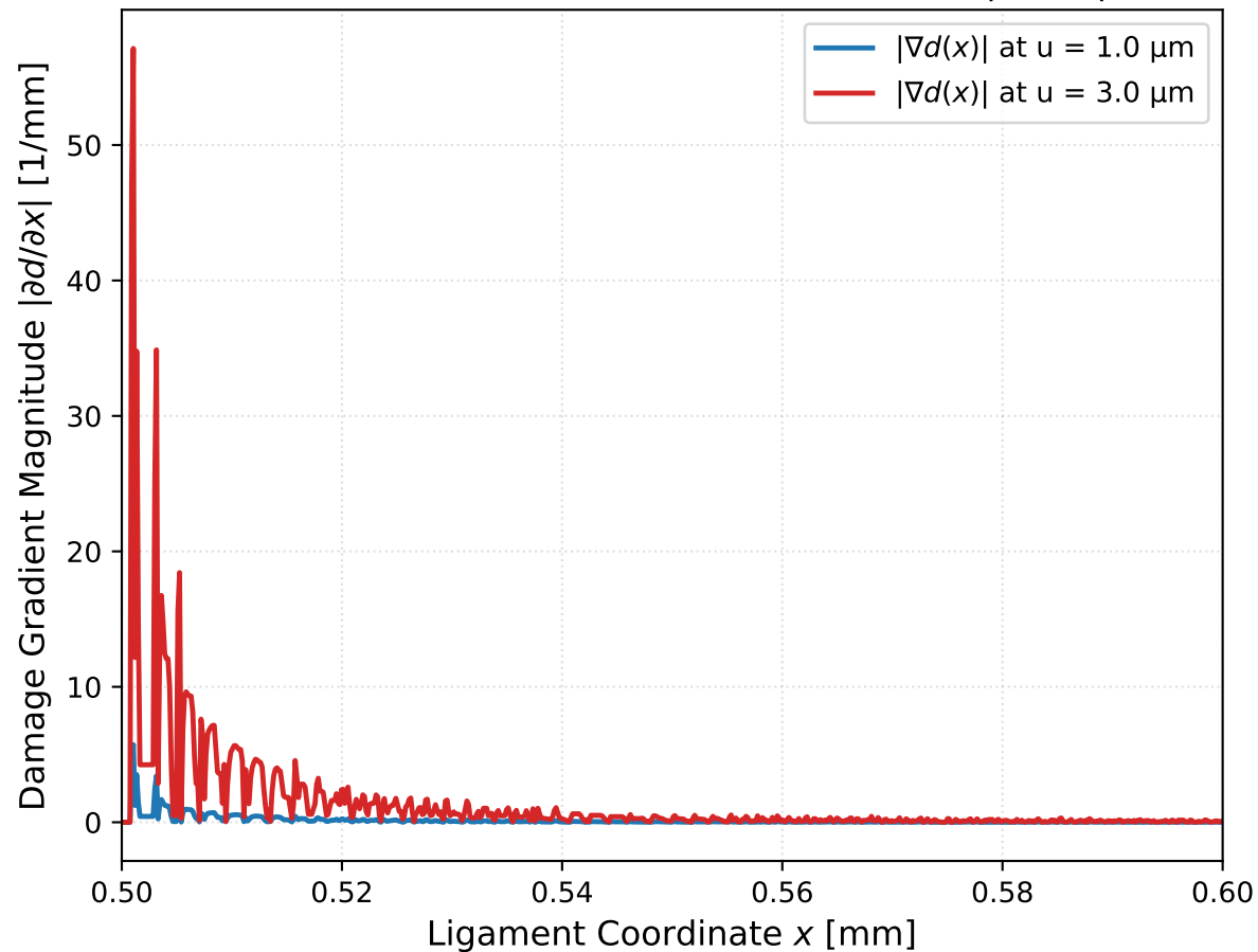
Phase-Field Localization Gradient Profile |\nabla d(x)|
