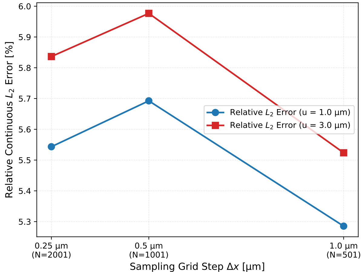
Grid Resolution Invariance: Relative L_2 Norm
