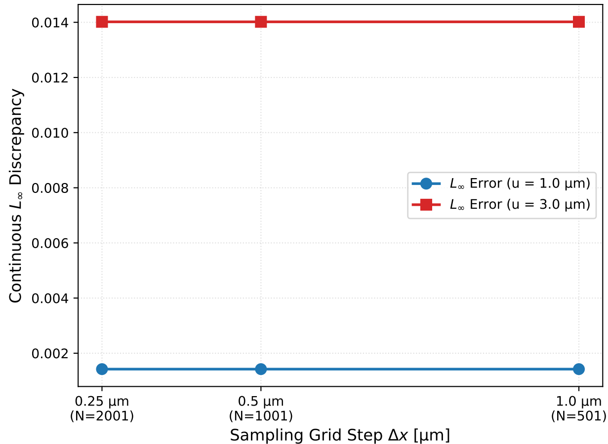
Grid Resolution Invariance: L_\infty Peak Norm
