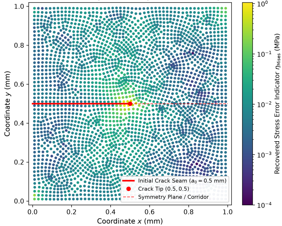
Figure 3.1: Canonical Mode-I Coarse Mesh MISESERRI Distribution (N_{\text{elem}} = 2,906, 5,812 \text{ Duplicate-Collapsed Values, Abaqus 2023})
