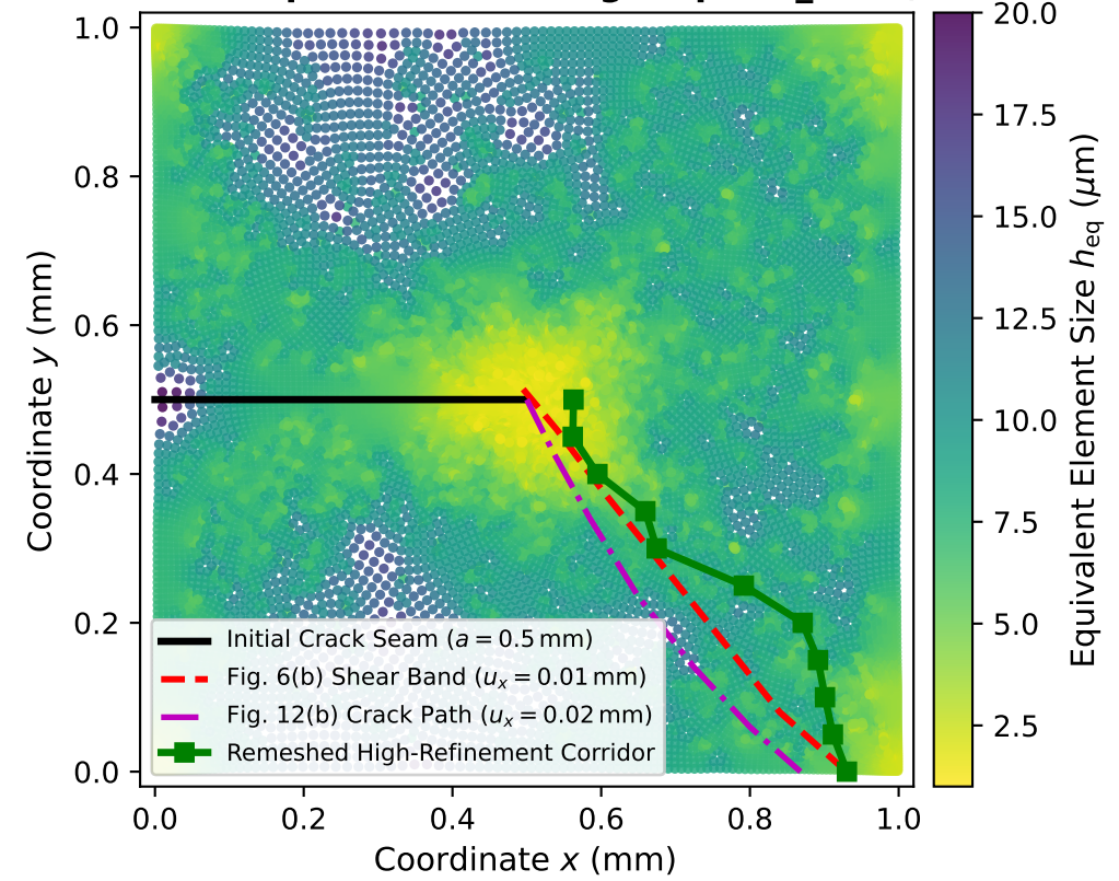
(b) Adapted Mesh Sizing Map (ET_2PCT, 22530 FEs)
