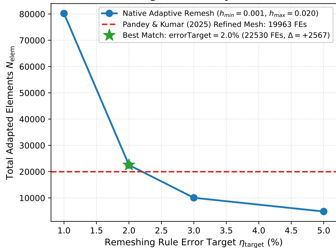
(a) OFAT Error Target Sensitivity vs. Publication Baseline
