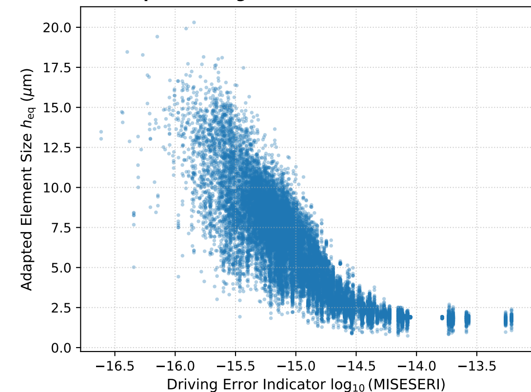
(c) Adaptive Sizing Inverse Correlation: r = -0.820
