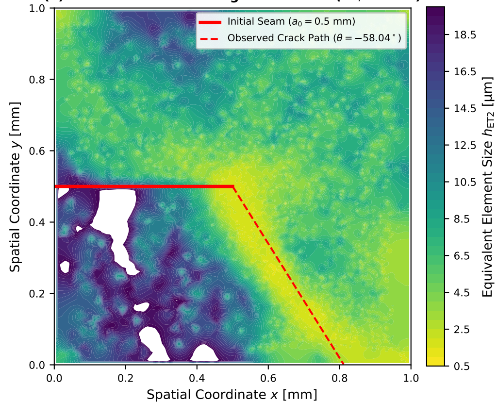
(a) Native ET2 Mesh Sizing Distribution (37,575 FEs)
