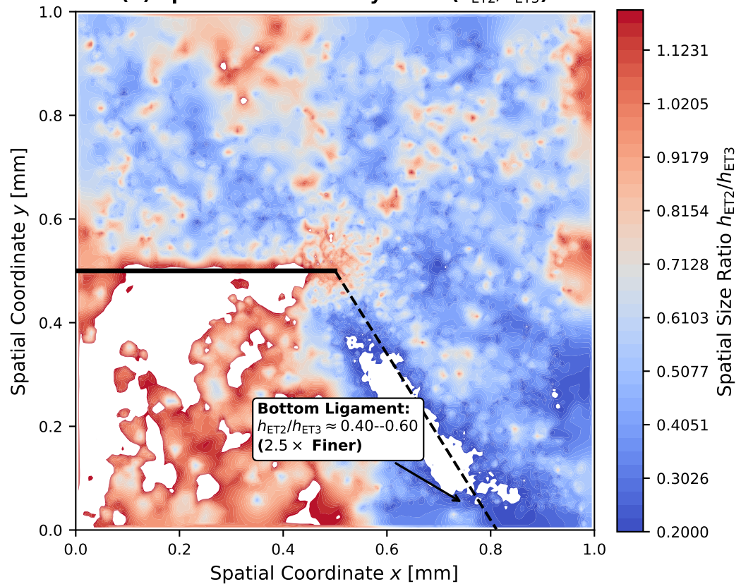
(b) Spatial Mesh Density Ratio ( h_{ET2}/h_{ET3} )
