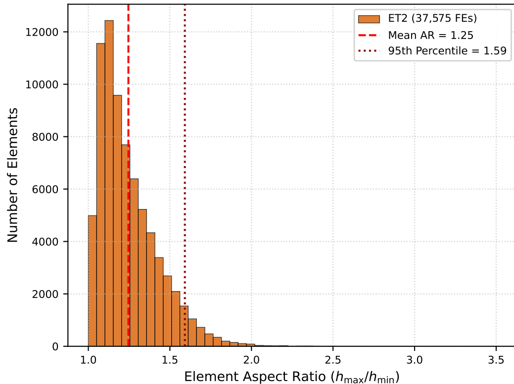
(a) Native ET2 Mesh Quality & Element Aspect Ratio
