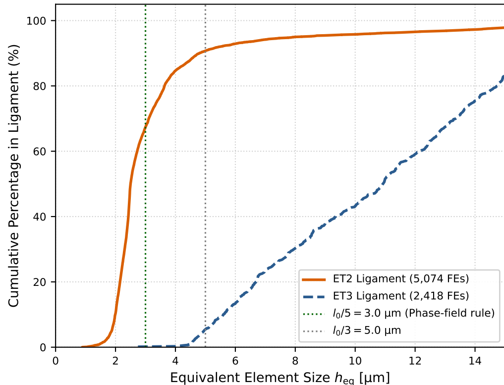
(b) Cumulative Element Sizing CDF in Ligament ( y \leq 0.10 mm)
