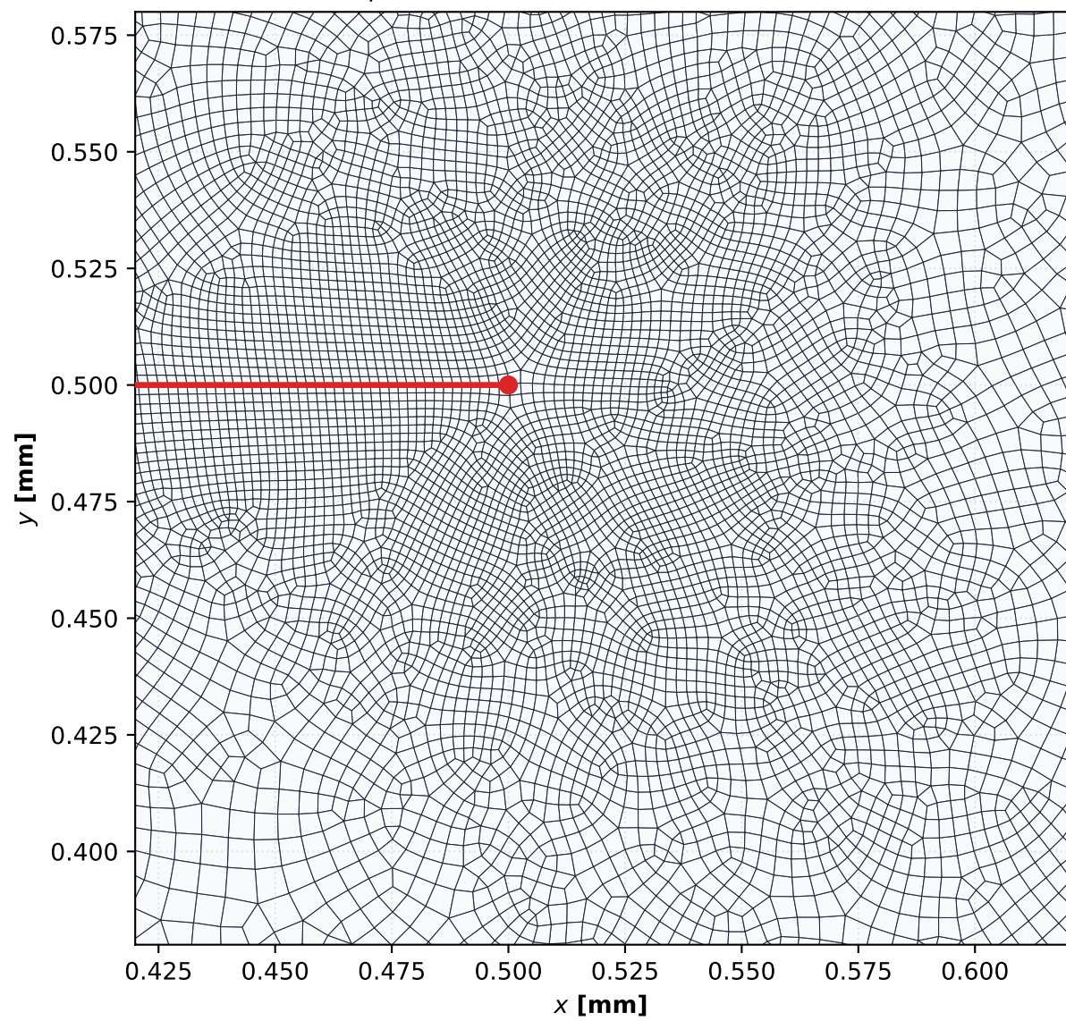
(c) Step-1 Crack-Tip Singularity Zoom
