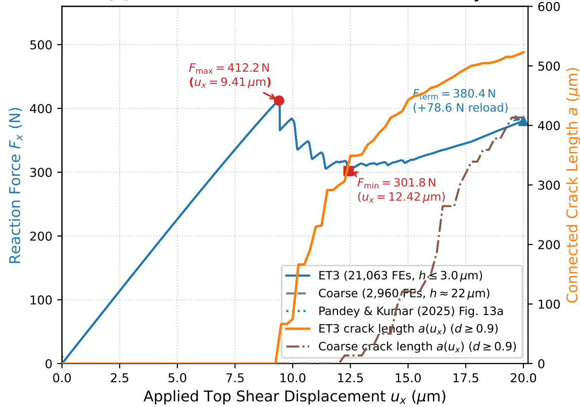
(a) Reaction Force & Crack Extension History
