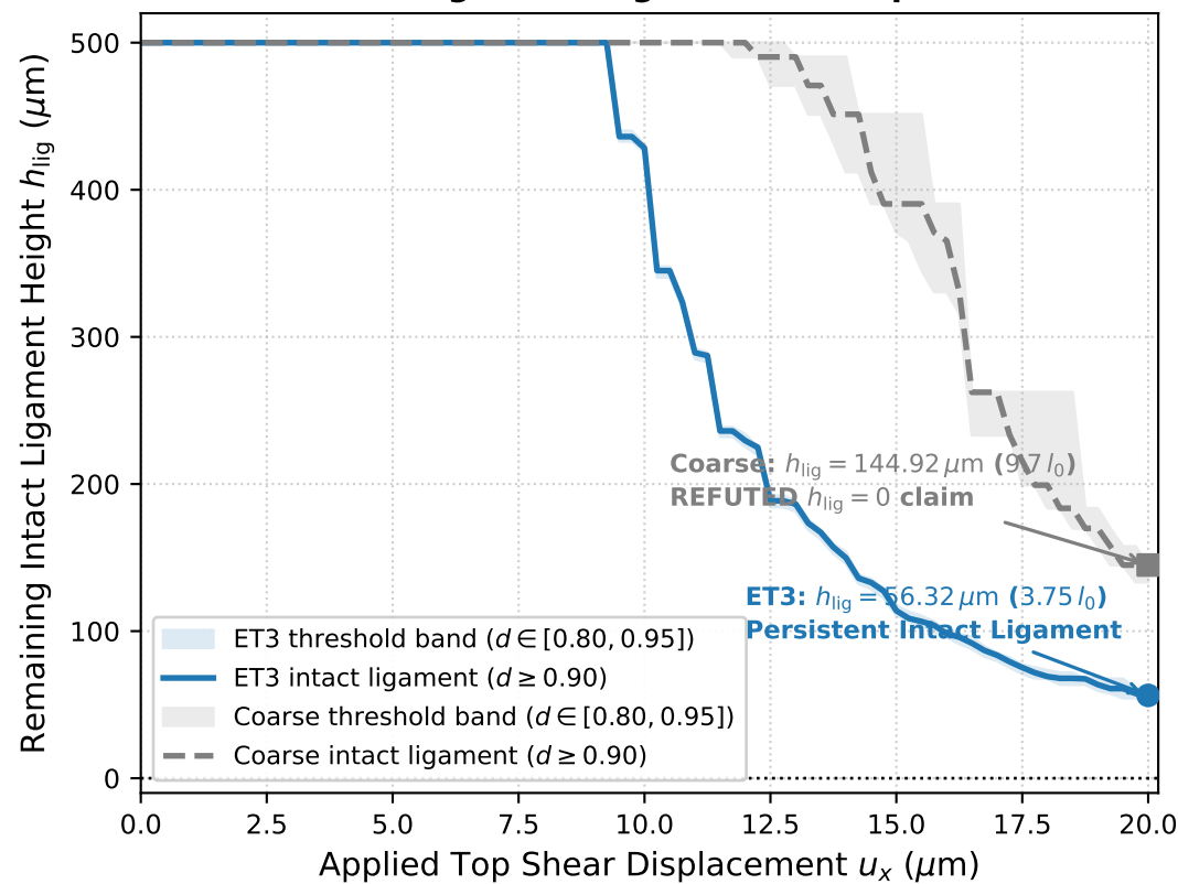
(c) Remaining Intact Ligament vs Displacement
