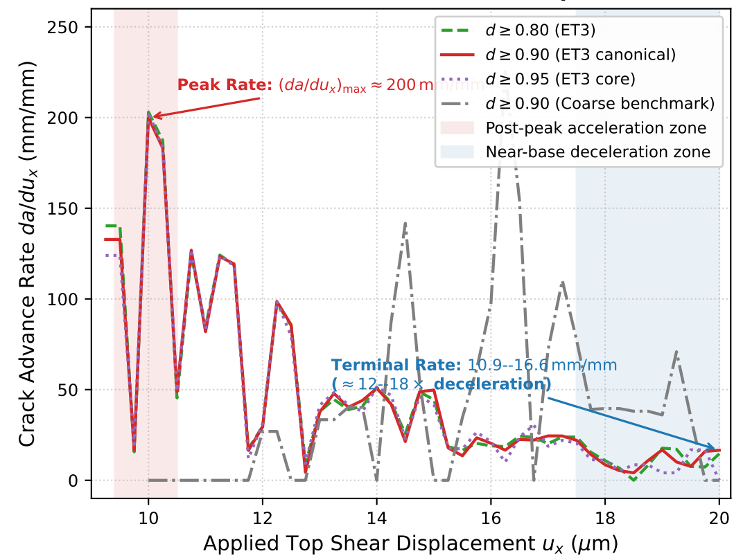
(b) Crack Advance Rate da/du_x vs Displacement
