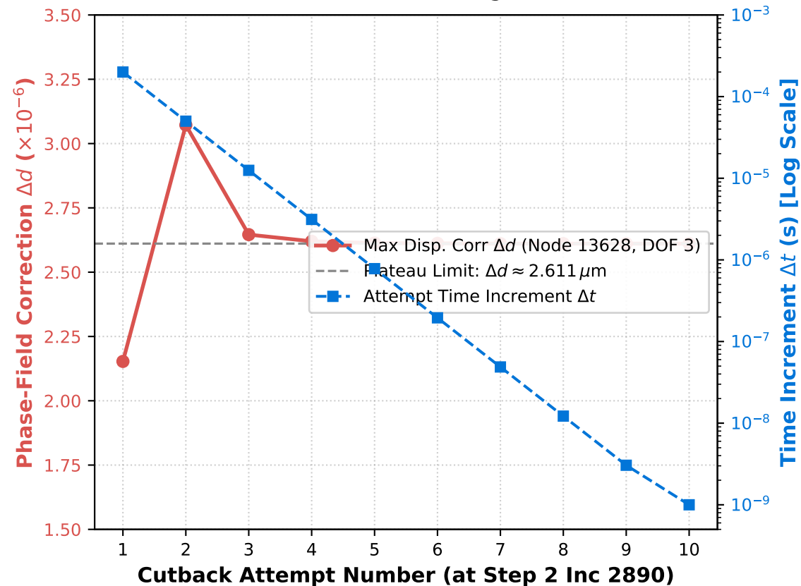
(a) Phase-Field Correction Stagnation Plateau
