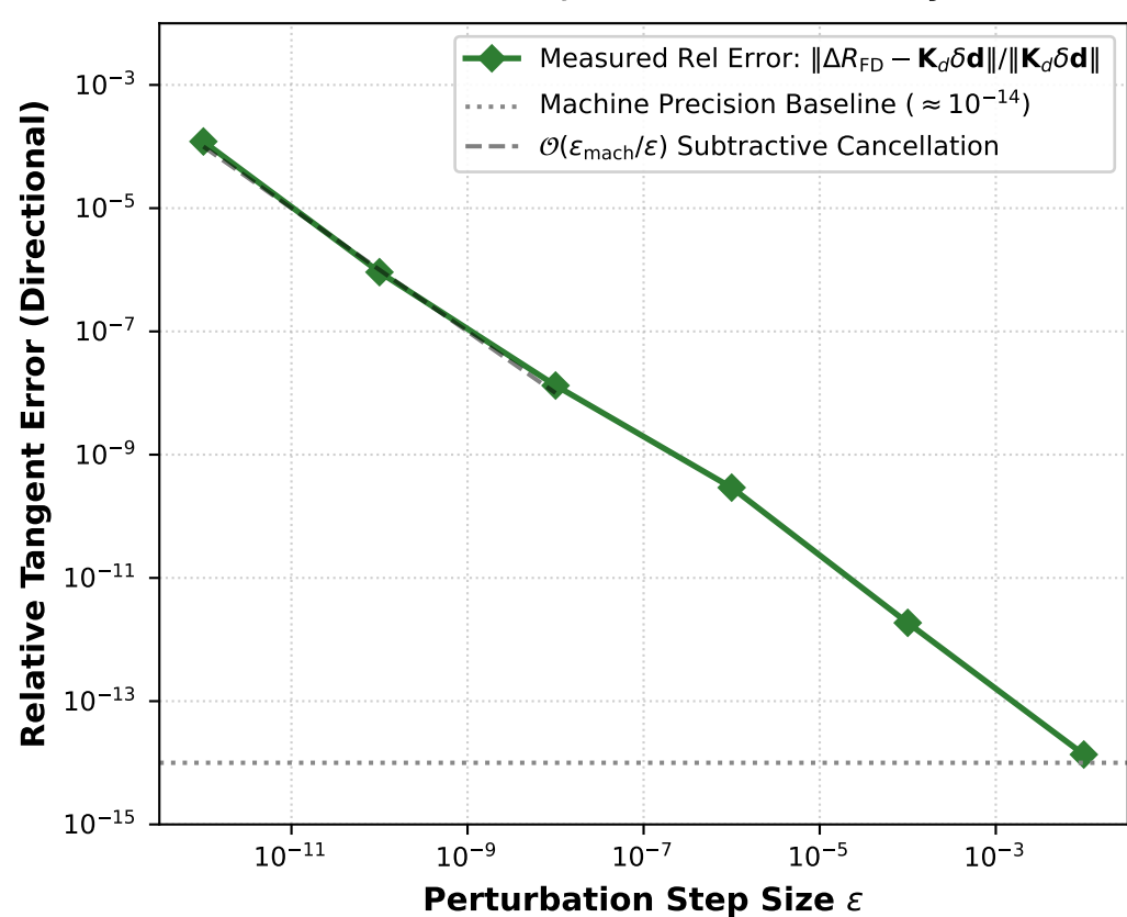
(b) Element-Level Jacobian Consistency Proof
