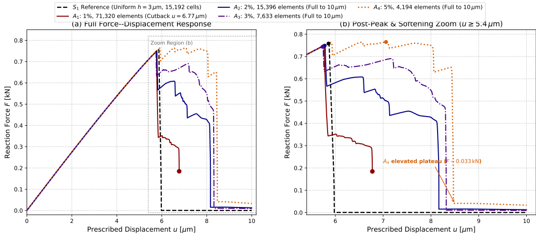
Fig. 4.8.: Force–displacement response of the canonical uniform reference S_1 and native adaptive meshes A_1 – A_4 : (a) full response over u \in [0, 10] \mu\text{m} ; (b) post-peak zoom over u \in [5.4, 10] \mu\text{m} . Production adaptive meshes contain 71,320, 15,396, 7,633, and 4,194 underlying finite elements for errorTarget values of 1%, 2%, 3%, and 5%, respectively. A_1 terminates at u = 6.77 \mu\text{m} , whereas A_2 – A_4 reach 10 \mu\text{m} .
