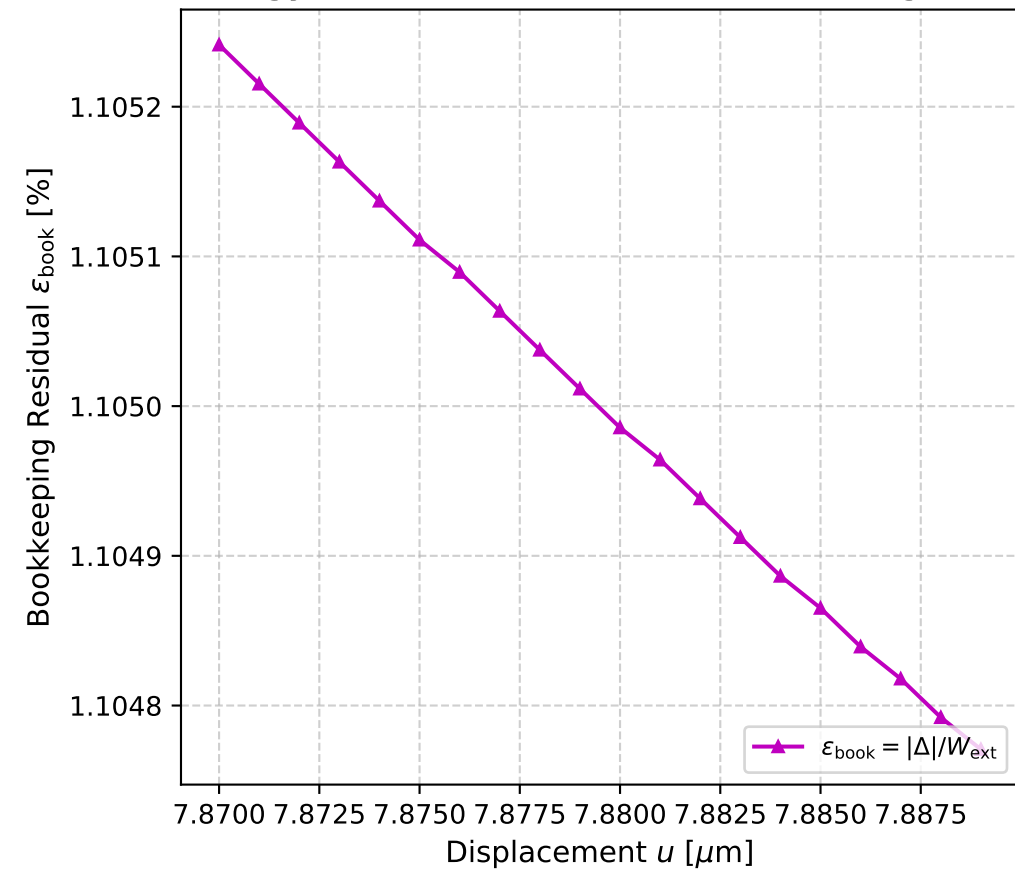
(c) Energy Balance Residual across Crossing Window
