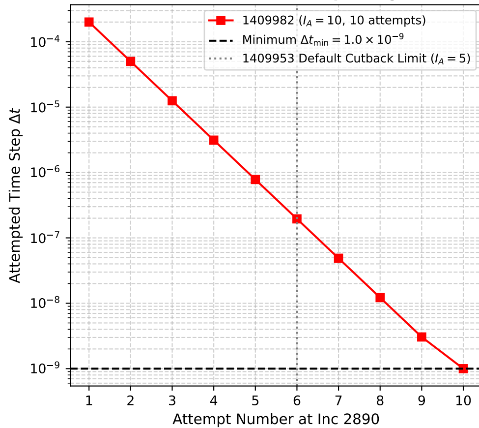
(b) Inc 2890 Cutback Attempt Progression
