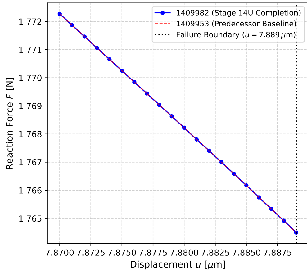
(a) Post-Peak Reaction Force near Failure Boundary
