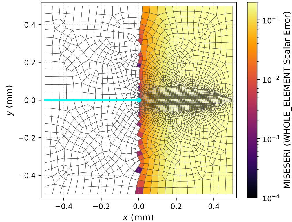
(a) Spatial MISESeri Field on 3,930 CPE4 Coarse Mesh
