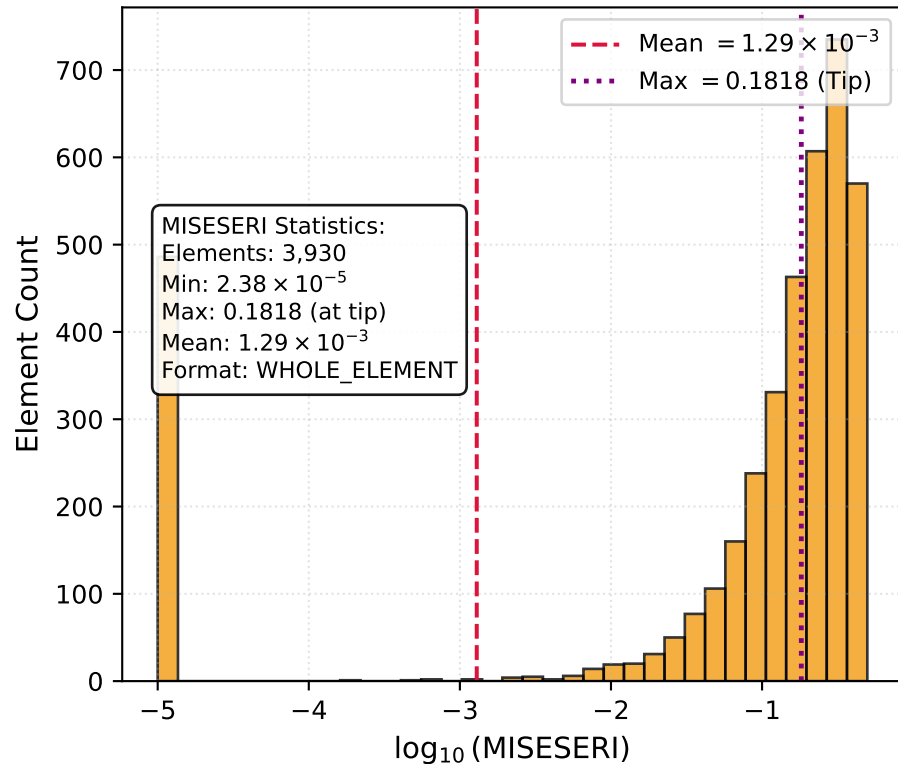
(b) Statistical Distribution of MISESeri Error
