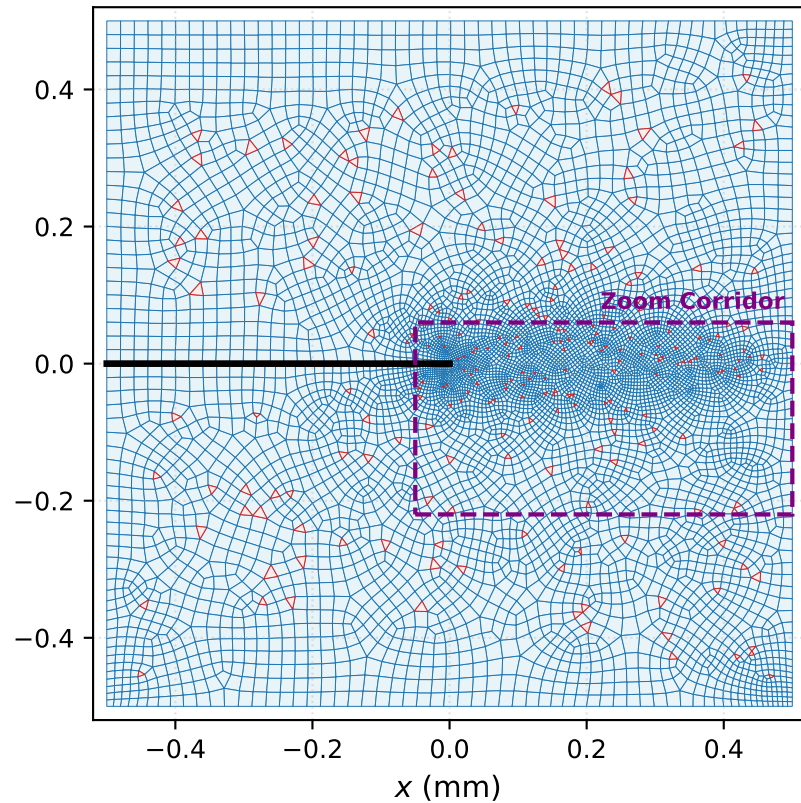
(a) Full Adaptive Domain (7,865 Finite Elements)
