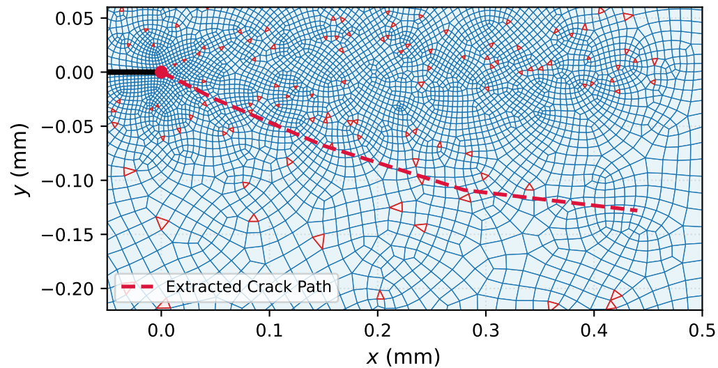
(b) Crack Zone Detail ( h_{\min} = 2.1 \mu\text{m} , Hybrid Quads/Tris)
