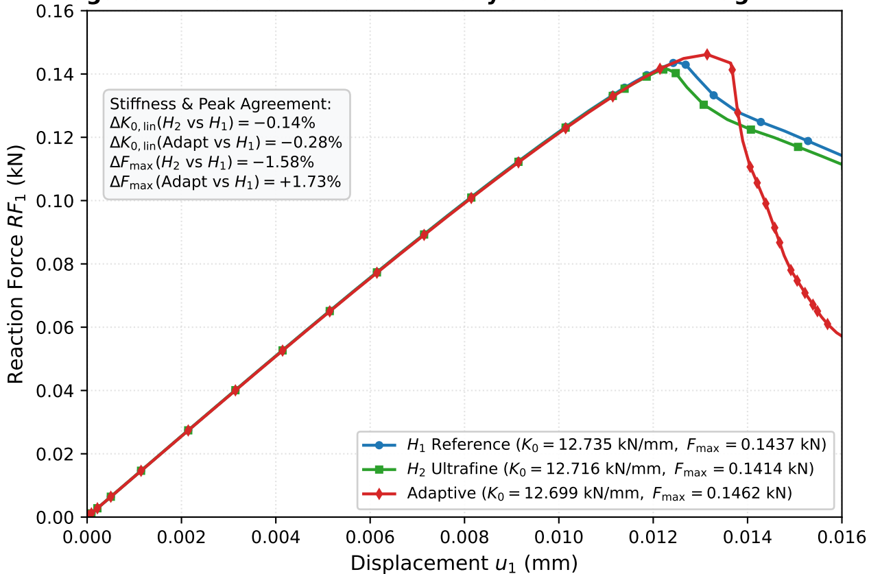
Figure 6: Pre-Peak Linear Elasticity and Peak Load Magnification
