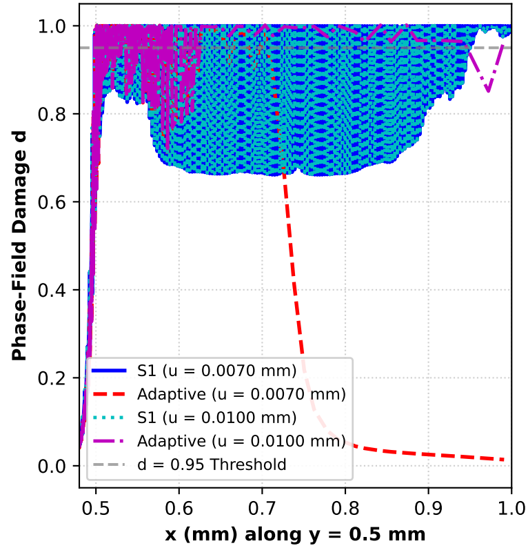
(a) Midplane Damage Profiles d(x, y = 0.5)
