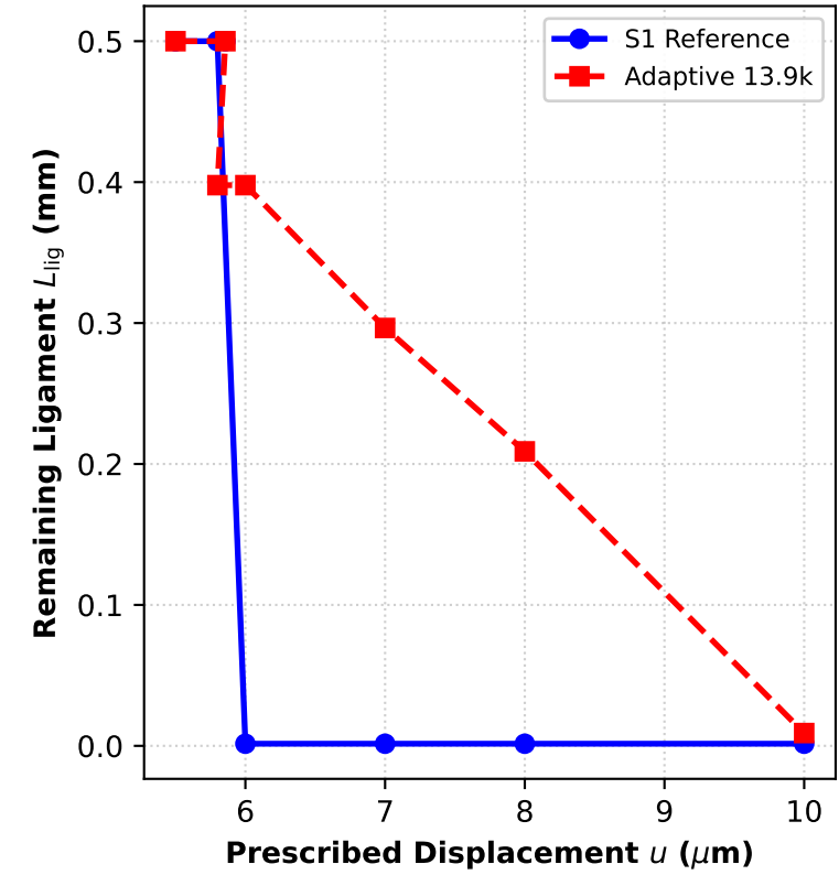
(c) Intact Ligament Length L_{\text{lig}}(u)
