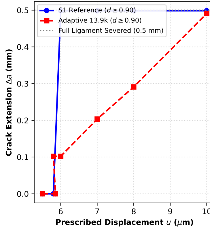
(b) Horizontal Crack Extension \Delta a(u)
