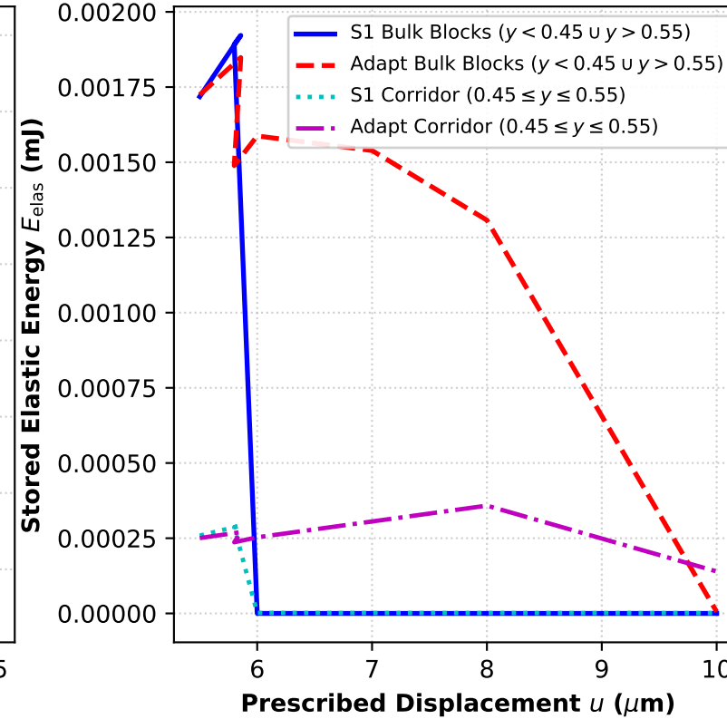
(e) Regional Elastic Strain Energy Partition
