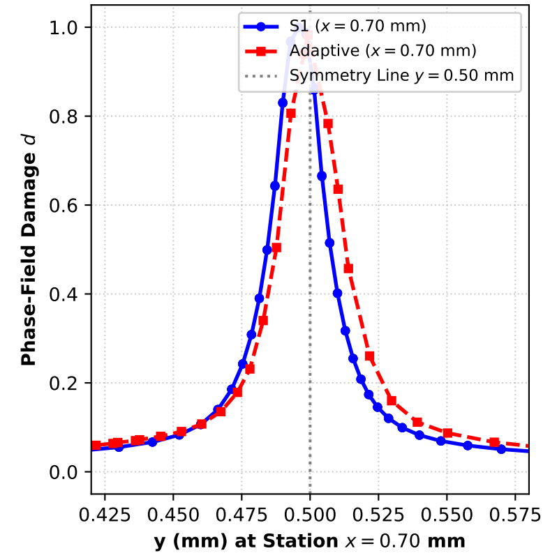
(f) Localization Profile d(y) at x = 0.70 mm
