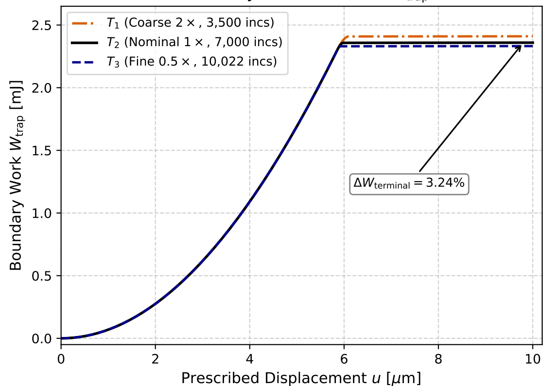
(a) Boundary Work Evolution W_{\text{trap}}(u)
