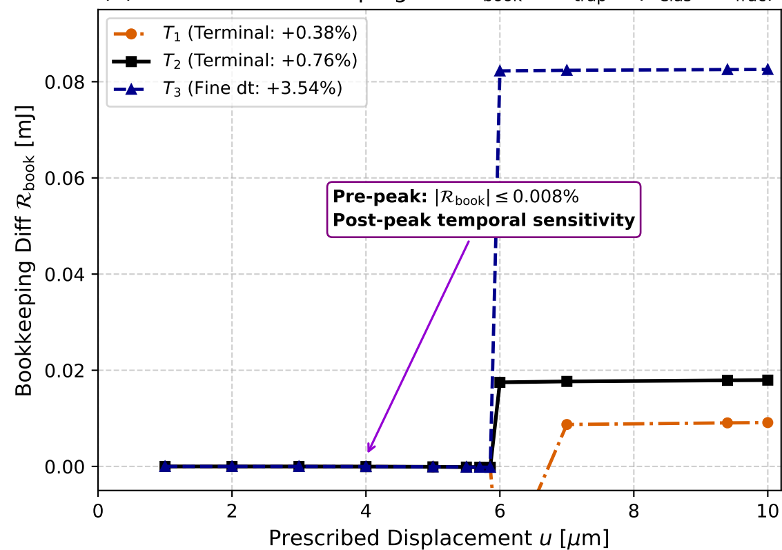
(d) Two-Term Bookkeeping Diff \mathcal{R}_{\text{book}} \equiv W_{\text{trap}} - (E_{\text{elas}} + E_{\text{frac}})
