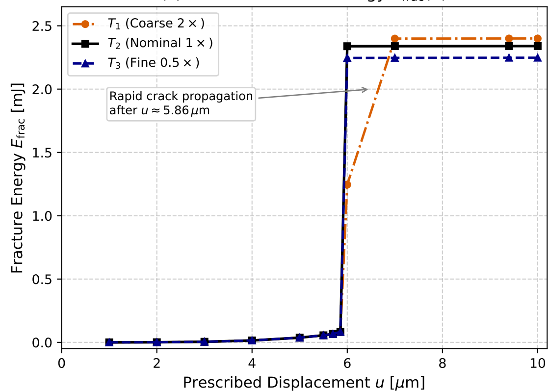
(c) Fracture Surface Energy E_{\text{frac}}(u)
