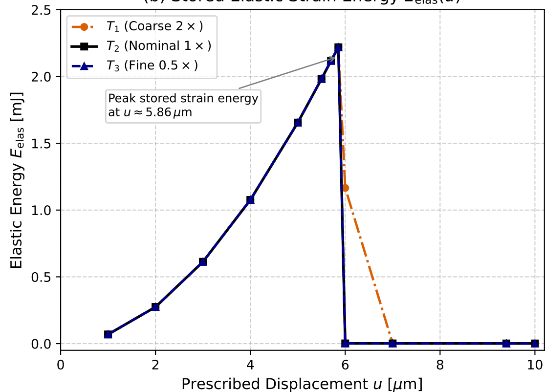
(b) Stored Elastic Strain Energy E_{\text{elas}}(u)
