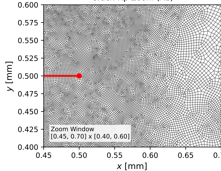
Crack-Tip Zoom (A1)
