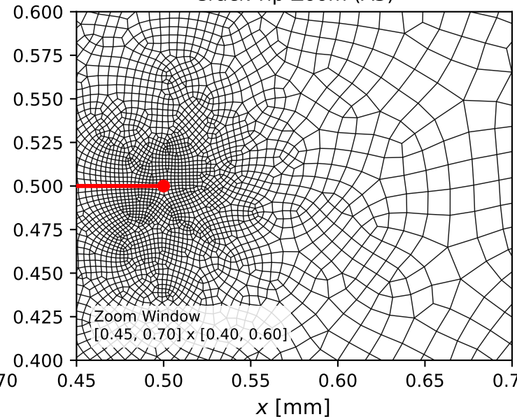
Crack-Tip Zoom (A3)
