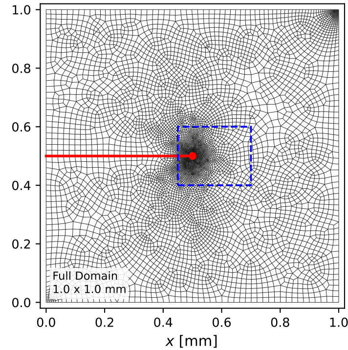
A_3 (3% Target Error) 7,633 elements
