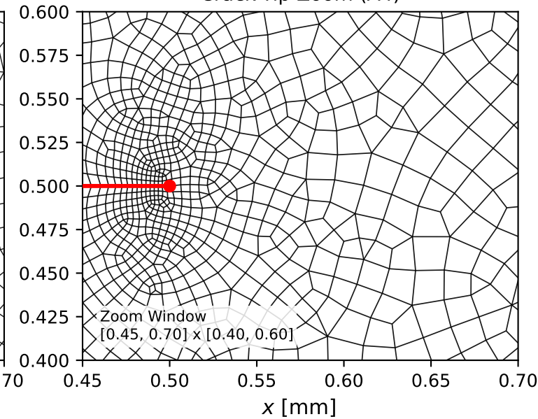
Crack-Tip Zoom (A4)
