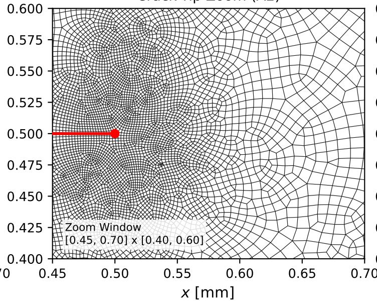
Crack-Tip Zoom (A2)
