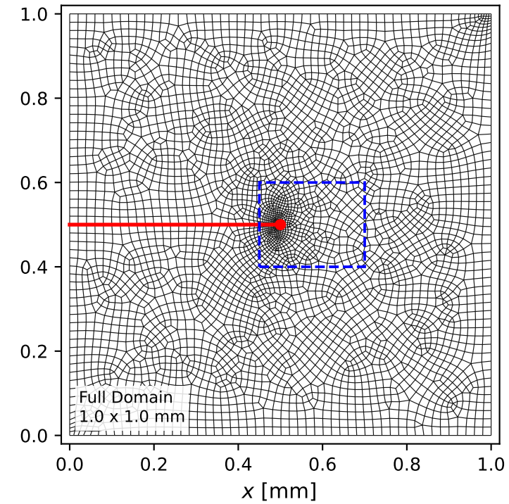
A_4 (5% Target Error) 4,194 elements
