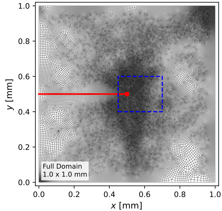
A_1 (1% Target Error) 71,320 elements
