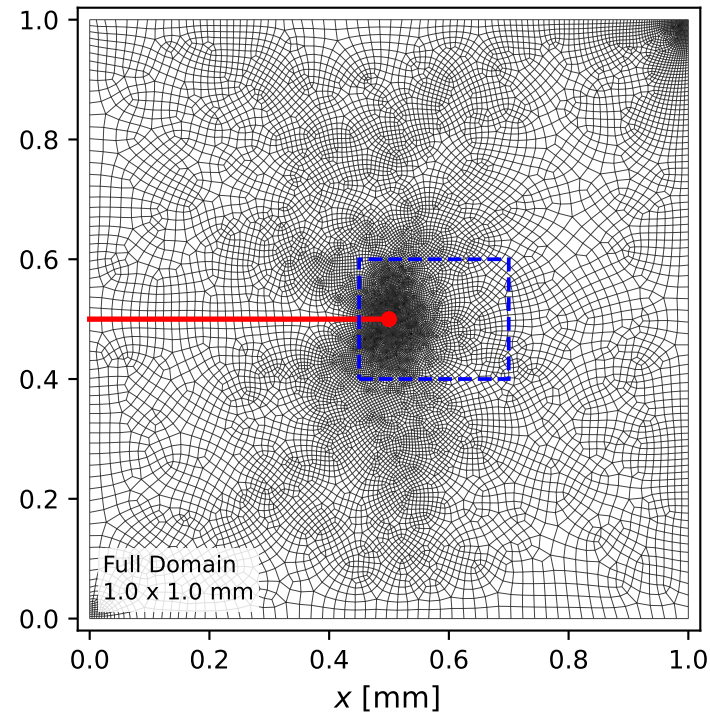
A_2 (2% Target Error) 15,396 elements
