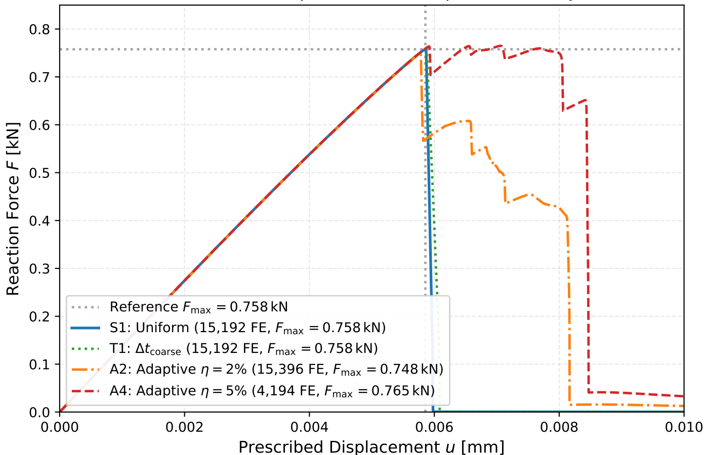
Mode-I Mechanical Response: Force-Displacement Trajectories
