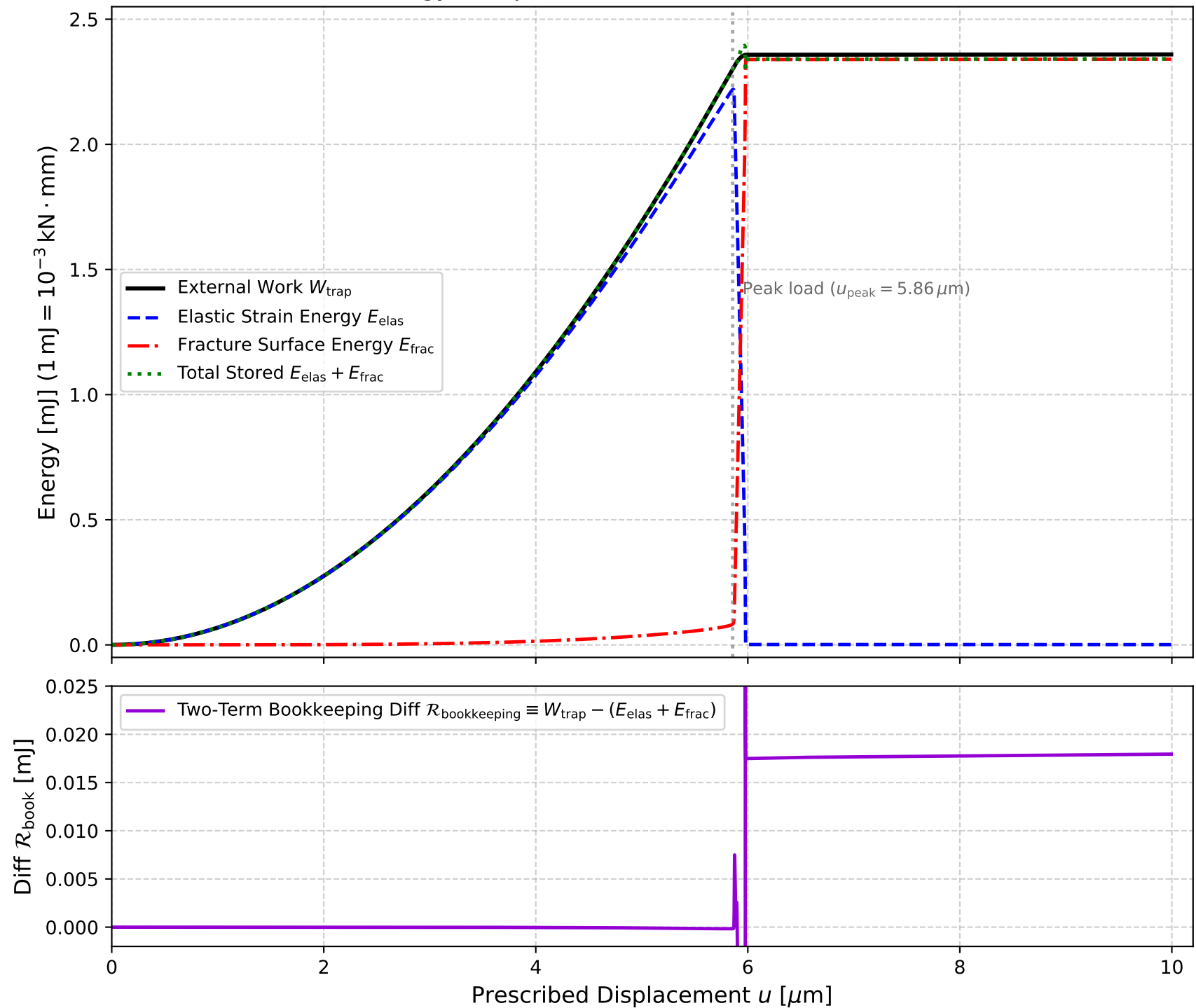
Global Energy Component Evolution (Baseline S1 / T2 Series)
